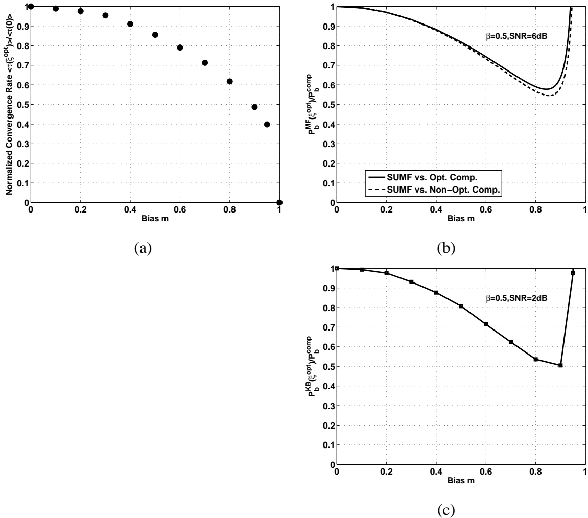
Fig. 3. (a) Normalized average convergence rate, \langle \tau(\xi^{opt}) \rangle / \langle \tau(0) \rangle , as a function of the bias m (for 1500 simulated systems). (b) SUMF BER comparison for the proposed scheme versus optimal and non-optimal (i.e., 5% above the entropy) compression as a function of bias m ( \beta = 0.5 and SNR = 6dB ). (c) Simulated BER comparison of Kabashima's detector for the proposed modification versus optimal compression as a function of bias m ( \beta = 0.5 and SNR = 2dB ). The squares denote simulation results, while the lines are only guides to the eye.
