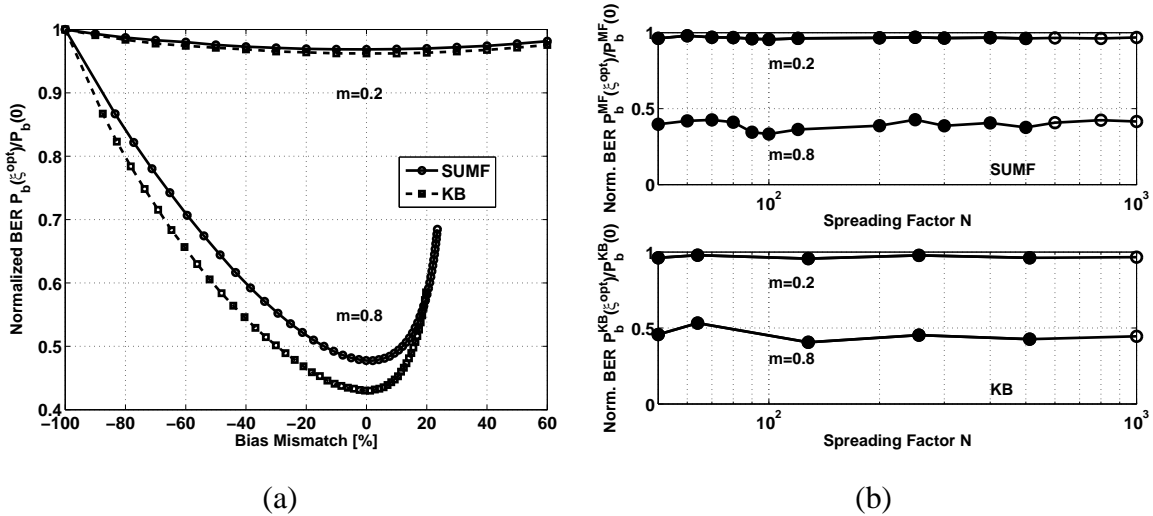
Fig. 2. (a) Simulated normalized BER, P_b(\xi^{opt})/P_b(0) , for the SUMF (circles and solid line) and Kabashima's multiuser (squares and dashed line) detectors as a function of the bias mismatch (in %) for both m = 0.2 (upper curves) and m = 0.8 (lower curves). Averaged over 10^4 simulated systems. (b) Normalized BER for SUMF (upper curves) and Kabashima's (lower curves) detectors as a function of the spreading factor N for both m = 0.2 and m = 0.8 ( 10^4 simulated systems). Full circles denote practical N values. In both figures, the lines are guides to the eye.
