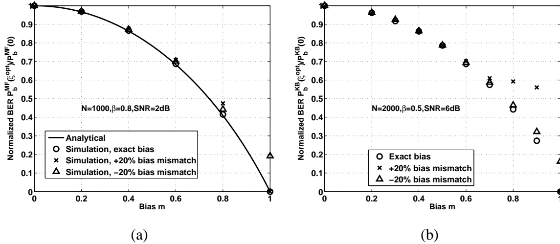
Fig. 1. (a) Normalized BER, P_b^{\text{MF}}(\xi^{\text{opt}})/P_b^{\text{MF}}(0) , for the SUMF detector as a function of the bias m for N = 1000 , \beta = 0.8 and \text{SNR} = 2\text{dB} . Analytical BER (solid line), computed according to expression (6), is compared to simulated BER (circles) assuming the exact source bias is known to the receiver. Also drawn ( \times and \Delta -marks) are the simulated BER curves under bias mismatch of \pm 20\% . Simulation results are averaged over 4000 systems. (b) Simulated normalized BER, P_b^{\text{KB}}(\xi^{\text{opt}})/P_b^{\text{KB}}(0) , for Kabashima's (KB) near-optimal detector [7] as a function of the bias m for N = 2000 , \beta = 0.5 , \text{SNR} = 6\text{dB} and averaged over 2000 systems. Simulated BER assuming exact bias (circles) knowledge at the receiver is compared to BER achieved under bias mismatch of \pm 20\% ( \times and \Delta -marks).
