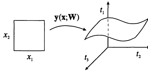
Figure 1: The latent variable density model constructs a distribution function in t -space in terms of a non-linear mapping \mathbf{y}(\mathbf{x}; \mathbf{W}) from a latent variable \mathbf{x} -space.
