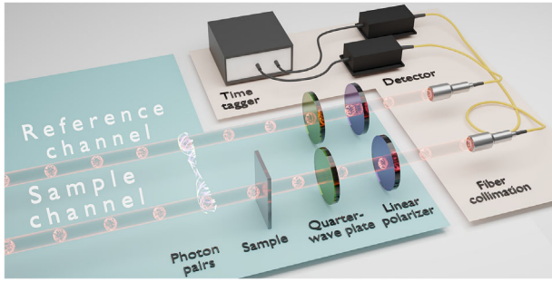
FIGURE 1 | Studied scenario of polarization-entangled photons scattering in a turbid medium. One of the photons of polarization-entangled photon pair interacts with a turbid sample. Another photon remains unchanged. Quarter-wave plates and linear polarizers enable polarization projective measurements. Coincidences between the channels upon photon detection are used for two-photon state reconstruction (Materials and Methods).
