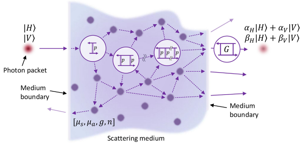
FIGURE 5 | Schematic representation of possible trajectories of the photon packets passing through a scattering medium. Notation |H\rangle and |V\rangle addresses the problem of entangled state modeling, where each trajectory can be followed by a photon packet with both horizontal |H\rangle and vertical |V\rangle polarization. In turn, \alpha_H|H\rangle + \alpha_V|V\rangle and \beta_H|H\rangle + \beta_V|V\rangle correspond to the resultant polarization states for initial either |H\rangle or |V\rangle input states. \mu_s , \mu_a , g , and n define the properties of the medium: scattering coefficient, absorption coefficient, scattering anisotropy factor, and refractive index, correspondingly [67]. One of the trajectories features ladder diagrams for visualization of the iterative solution of the Bethe-Salpeter equation. Here, G denotes the propagator of the Bethe-Salpeter equation and p stands for the scattering phase function (adapted from Ref. [62]).
