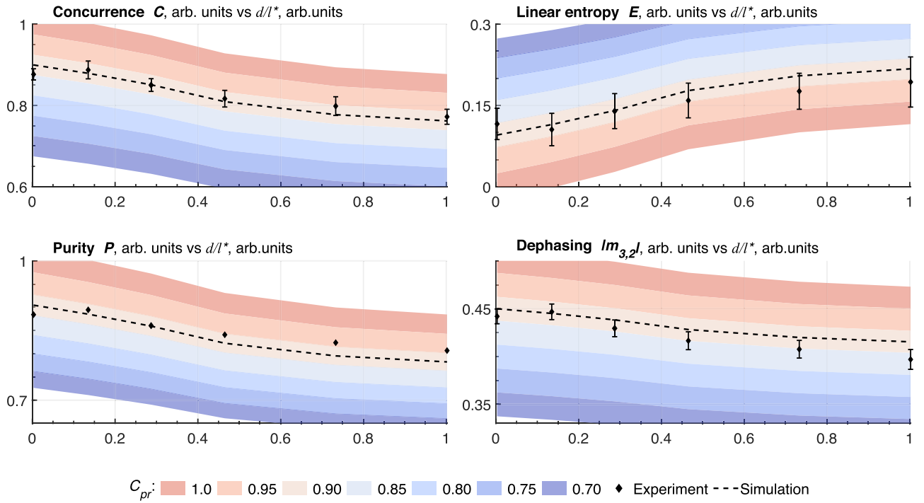
FIGURE 4 | Evolution of the polarization-entangled two-photon state due to interaction with a scattering medium. Dependencies of the output state's concurrence, linear entropy, purity, and dephasing versus the effective thickness of the scattering medium d/l^* . Experimentally measured points (diamonds, C_{pr} = 0.88 \pm 0.01 ) with error estimation [55] and simulated outcome with best fitting probing state (dashed line, C_{pr} = 0.90 ) for d/l^* = 0.003, 0.135, 0.287, 0.465, 0.733 , and 1.002 . Shaded stripes show simulation results beyond experimentally realized conditions with different degree of entanglement of the initial probing state C_{pr} = 1.0, 0.95, 0.90, 0.85, 0.80, 0.75 , and 0.70 .
