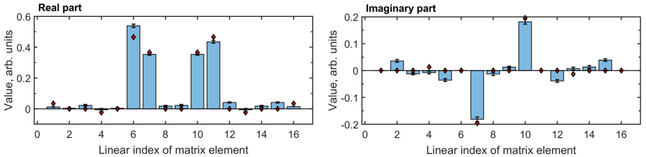
FIGURE 3 | Correlation between measured and modeled changes to the probing Bell state after interaction with a turbid sample. Measured (barplot) and modeled (diamonds) density matrix elements from Figure 2 reshaped to vectors. Error bars represent the error estimation as per Ref. [55].
