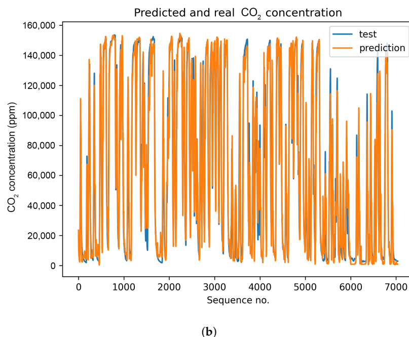
Figure 9. Vehicle onboard deployment. (a) Setup. (b) Prediction against real recorded values.
