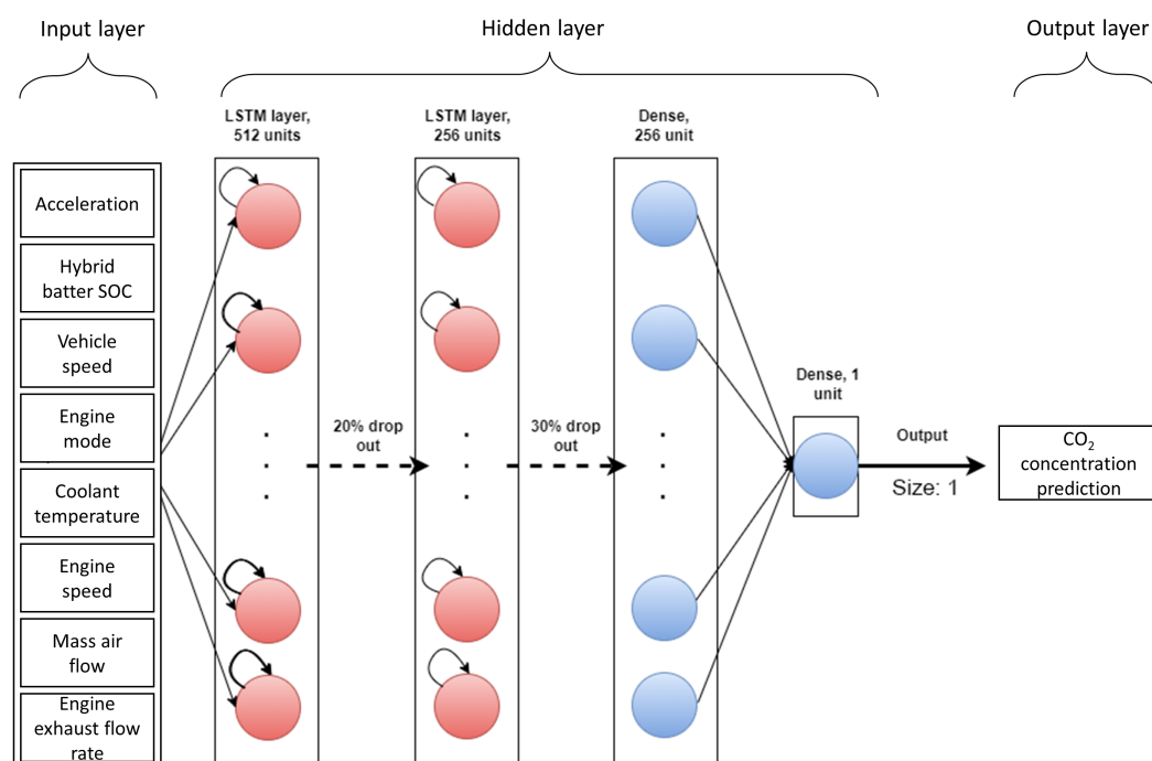
Figure 5. Architecture of proposed LSTM-based algorithm.
