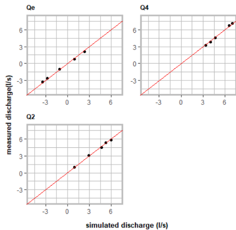
Fig. A1. Combined scenario pipe flows of configuration 1 - calibration data set.
