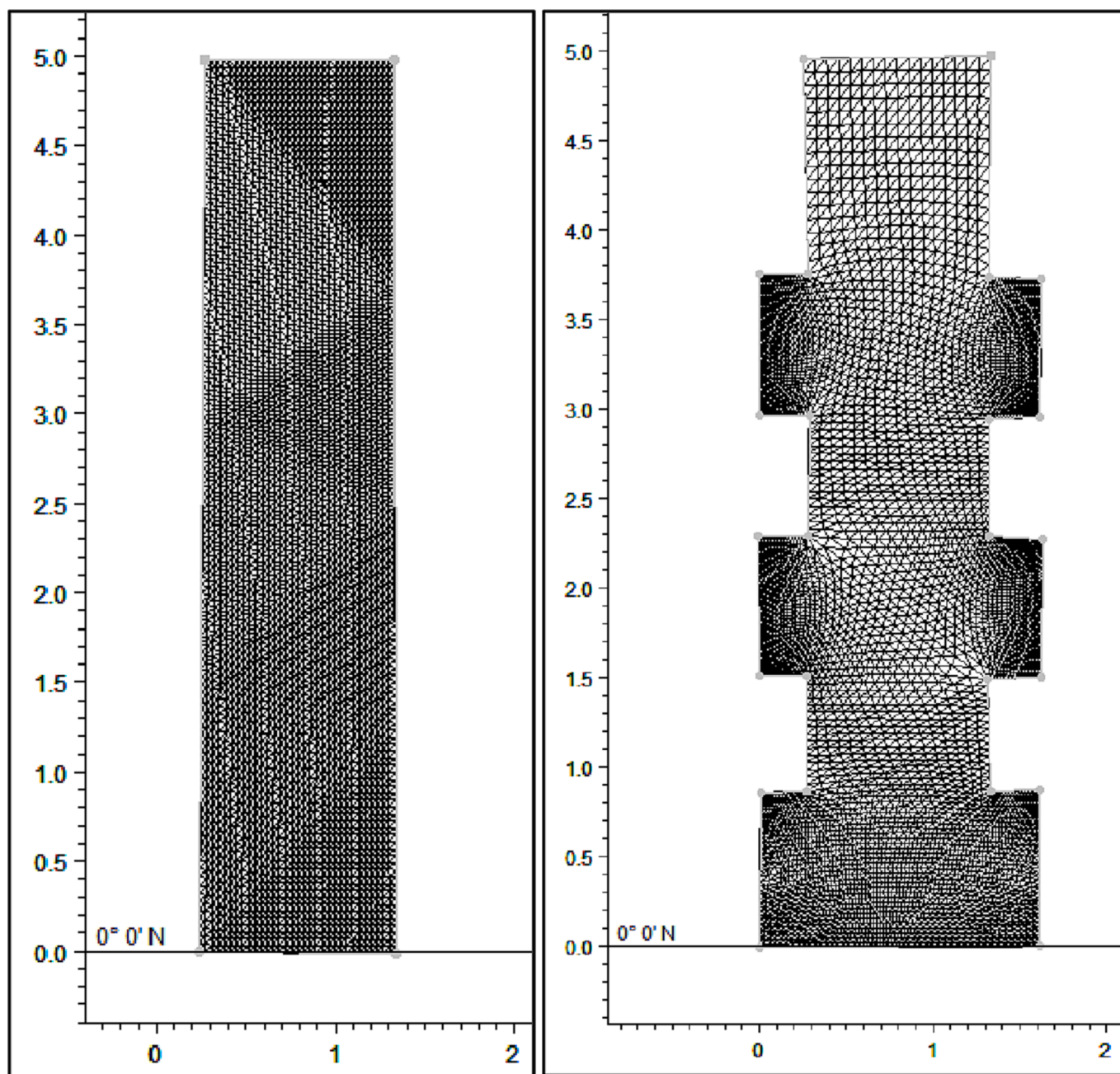
Fig. 4. The meshes used for each configuration. The left shows configuration 1 and the right shows configuration 2. Both have a geometry of 1 m \times 5 m.
