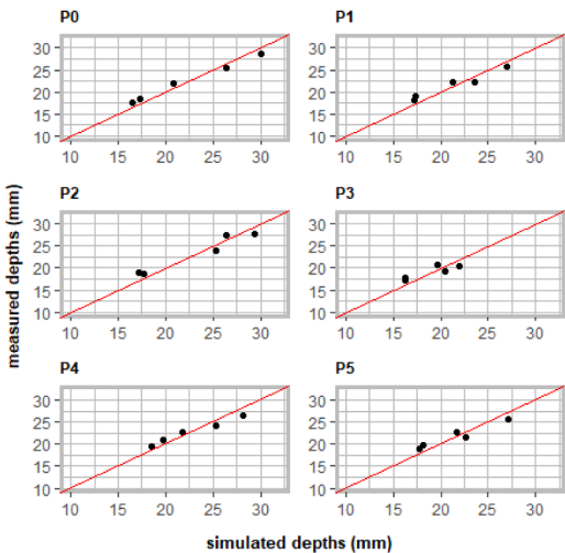
Fig. B1. Combined scenario surface depths of configuration 1- calibration data set.
