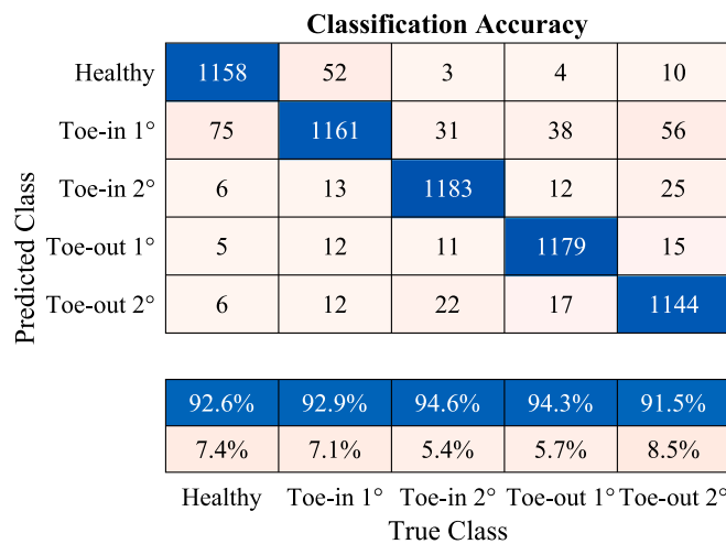
Fig. 21. Confusion matrix for different alignment conditions using SVM.
