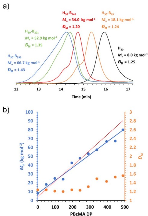
Fig. 3 DMF GPC data obtained for PHEMA 30 - b -PBzMA y block copolymers synthesised via RAFT dispersion polymerisation of benzyl methacrylate in [EMIM][DCA] at 15% w/w solids. GPC data was obtained against poly(methyl methacrylate) standards. (a) Chromatograms obtained for a selection of PHEMA 30 - b -PBzMA y block copolymers, where PHEMA is denoted as H and PBzMA is denoted as B. (b) M n vs. PBzMA DP (blue), where the blue line indicates the line of best fit, and D M vs. PBzMA DP (orange), where the red dashed line indicates the theoretical M n vs. PBzMA DP. Theoretical M n and DP were obtained by 1 H NMR spectroscopy, and actual M n and D M were obtained by GPC analysis.
