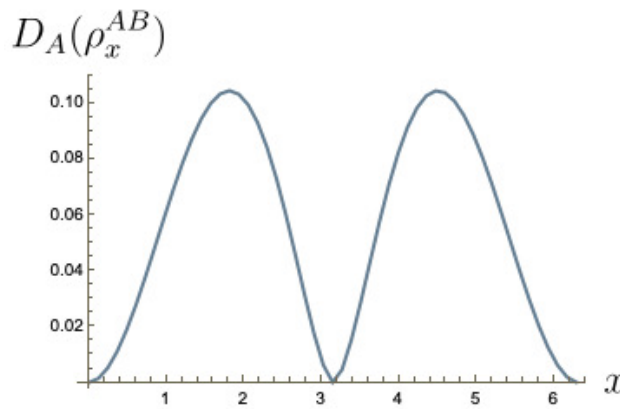
Figure 1: This shows the numerical discord for the state in Eq. (16). It is clear there is zero quantum correlation at x = 0, \pi . Elsewhere, there is non-zero quantum correlation, with the maximum occurring around x \approx n\pi + \pi/2 , where n \in \mathbb{Z} . The minimisation was over \theta , and \phi as defined in the projectors. This can only occur for a 2-qubit state, as the parameterisation for \theta and \phi is only valid for a two particle system. Note, \phi is included here for the optimisation to compute the discord, but for the optimisation in the game, \phi = 0 to allow analytical tractability.
