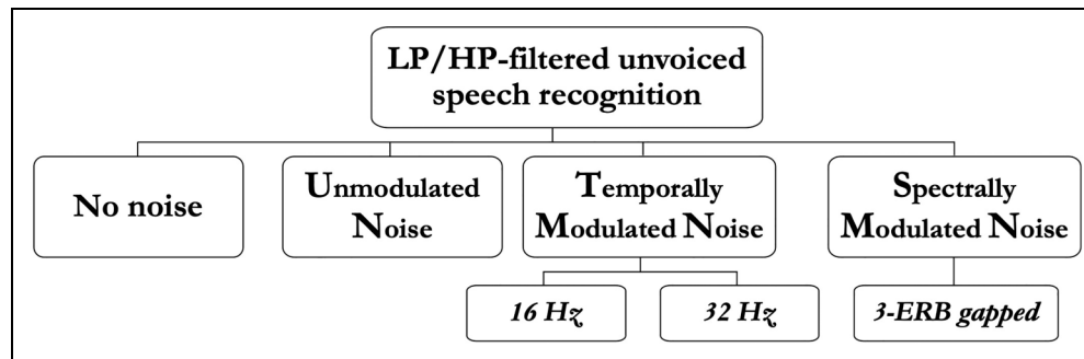
Figure 2. Tested conditions for unvoiced speech recognition task.
