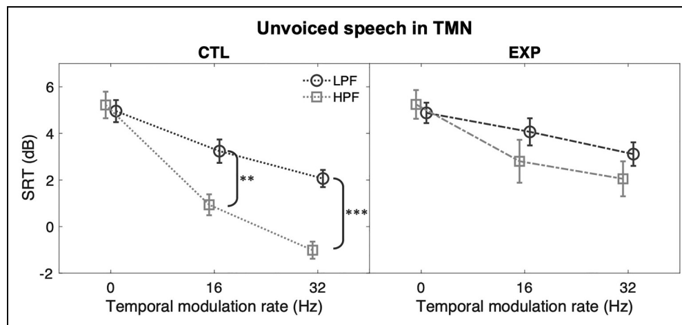
Figure 5. SRT differences between LPF (dark grey) and HPF (light grey) unvoiced speech in UN and TMNs within the CTL (left panel) and the EXP group (right panel). Error bars: SEM. *, p < 0.05 ; **, p < 0.01 ; ***, p < 0.001 .
