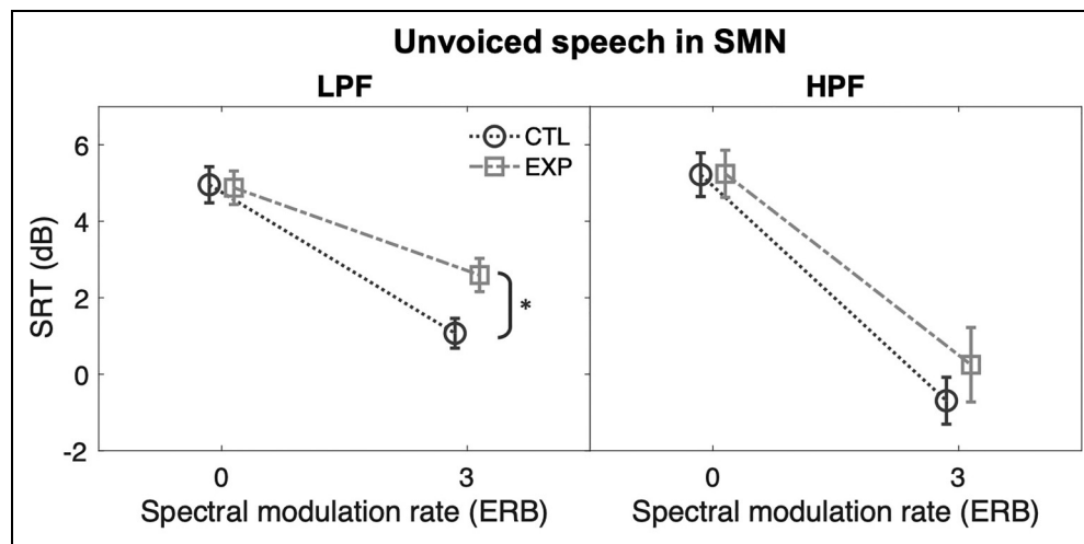
Figure 6. SRTs of unvoiced speech in SMN under LPF (left panel) and HPF (right panel) conditions. Error bars: SEM. *, p < 0.05 ; **, p < 0.01 ; ***, p < 0.001 .
