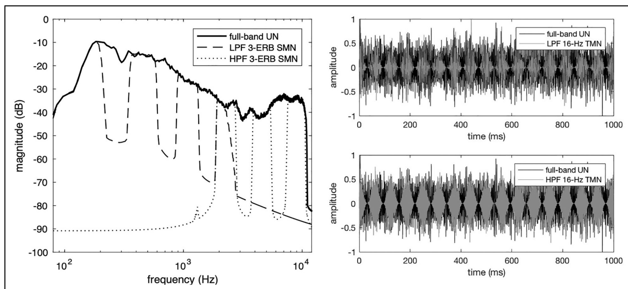
Figure 1. Left panel: spectra of the full-band unmodulated noise (solid), LPF SMN (dashed), HPF SMN (dotted). Right panel: time-domain waveforms of the full-band unmodulated noise (black), 16-Hz LPF TMN (top, grey), 16-Hz HPF TMN (bottom, grey).
