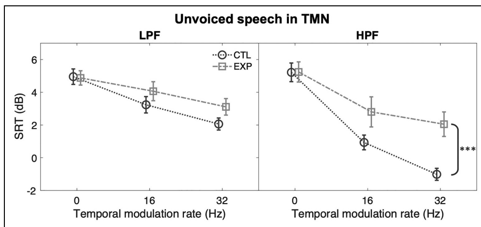
Figure 4. Difference between the CTL (dark grey) and the EXP (light grey) groups in SRTs of unvoiced speech in UN (0 Hz), 16-Hz and 32-Hz TMNs under LPF (left panel) and HPF (right panel) conditions. Error bars: SEM. *, p < 0.05 ; **, p < 0.01 ; ***, p < 0.001 .
