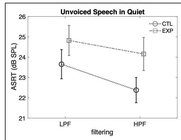
Figure 3. Performance of LPF and HPF unvoiced speech in quiet between the CTL (dark) and the EXP (light) groups. Error bars: the standard error of the mean (SEM).
