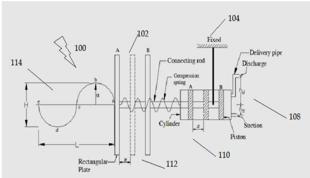
Fig.1: Schematic Diagram of a New Concept WEC.
