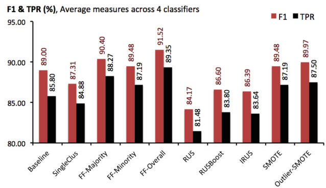
Fig. 4 Comparison of F1 and TPR scores obtained by examined methods, as averages across classification models and 30 trials of 10-fold cross validation
