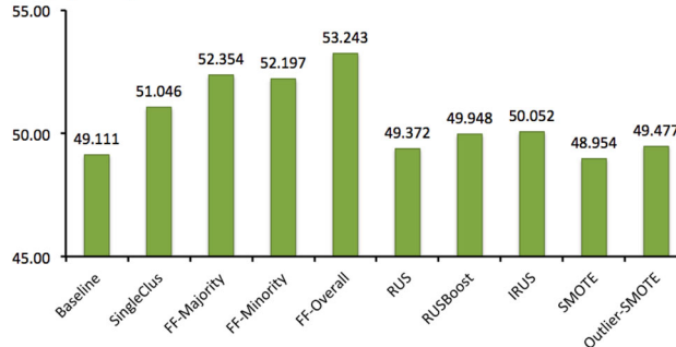
Fig. 6 Comparison of TPR scores obtained by different methods for classifying obfuscated instances. These are averages across classification models and 30 trials of tenfold cross validation
