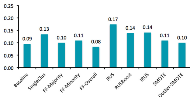
Fig. 5 Comparison of FPR scores obtained by examined methods, as averages across classification models and 30 trials of 10-fold cross validation
