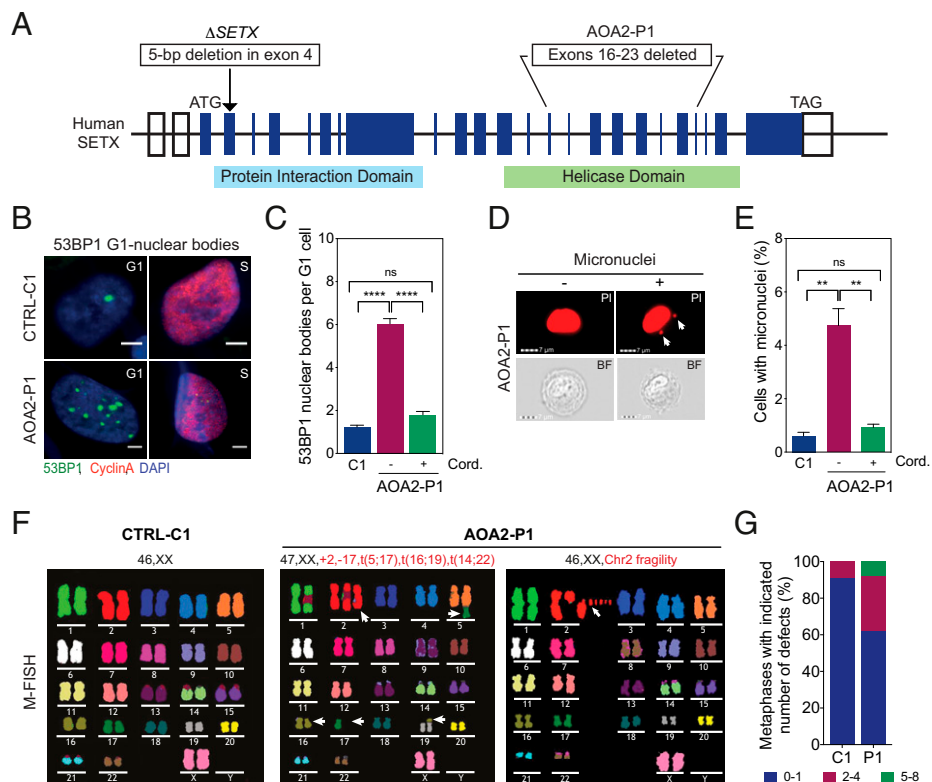
Fig. 1. SETX deficiency promotes chromosome fragility. (A) Diagram of human SETX showing \Delta SETX and the AOA2-P1 mutant fibroblasts. Boxes represent exons and the positions of start (ATG) and stop (TAG) codons. (B) Immunostaining with 53BP1 (green) and cyclin A (red) antibodies in control (CTRL-C1) and AOA2-P1 fibroblasts. DNA was stained with DAPI (blue). Representative images of G1- and S-phase cells are shown. (Scale bars, 5 \mu m.) (C) Quantification of 53BP1 NBs in G1 cells, as in B, with or without cordycepin. Data represent the mean \pm SEM of three independent experiments with >300 cells per condition. (D) Imagestream imaging flow cytometry of AOA2-P1 fibroblasts. Nuclei were stained with PI. Representative PI and bright field (BF) images of mononucleated cells with and without micronuclei are shown. White arrows denote micronuclei. (Scale bars, 7 \mu m.) (E) Quantification of cells with micronuclei, as in D. Cells were treated with or without cordycepin. Data represent the mean \pm SEM of three independent experiments, >4,000 cells per condition. (F) M-FISH analyses of metaphase spreads from CTRL-C1 and two AOA2-P1 fibroblasts showing deletions/amplifications and chromosome fragility. Representative karyotypes are shown. White arrows, chromosome aberrations. (G) Quantification of metaphases with indicated number of aberrations, as in F. Thirty metaphases were analyzed per condition. ** P < 0.01 and **** P < 0.0001 by Mann–Whitney U test. P \geq 0.05 is considered not significant (ns).
