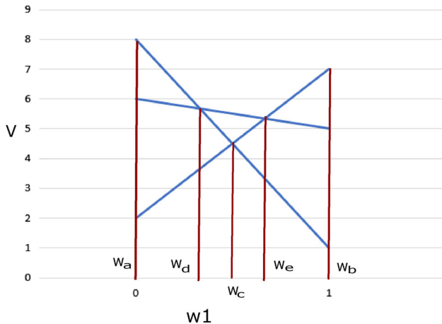
Fig. 3 Optimistic Linear Support
