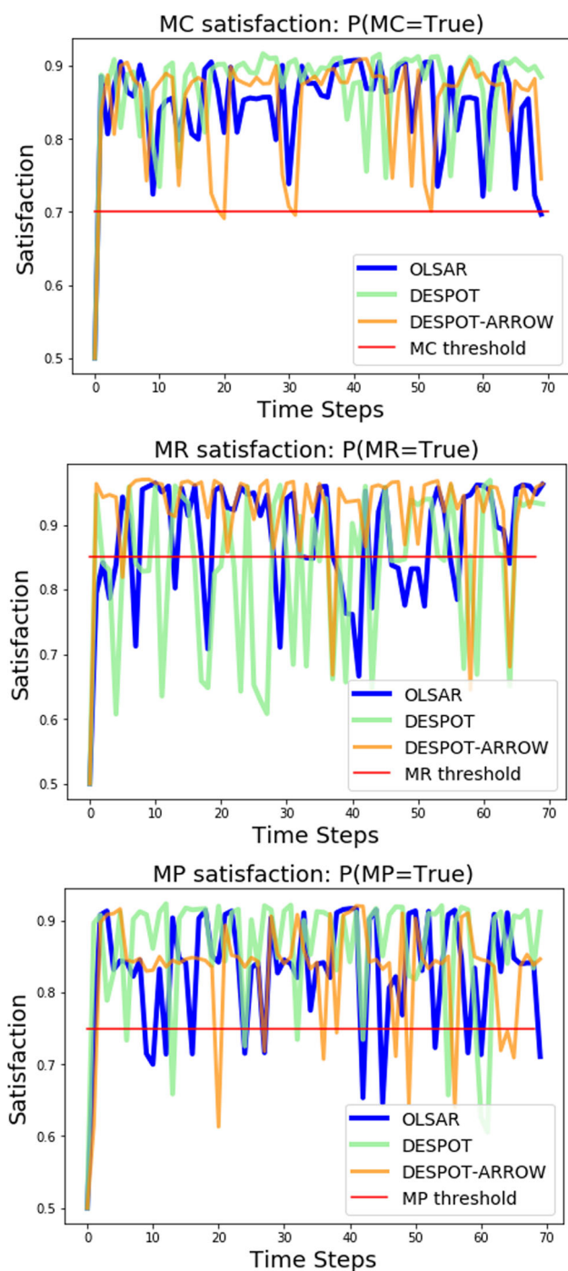
Fig. 12 Satisfaction of NFRs over time under detrimental context 2 (DC2) by applying Pri-AwaRE (using OLSAR), RE-STORM (using DESPOT) and RE-STORM-ARROW (using DESPOT-ARROW)
