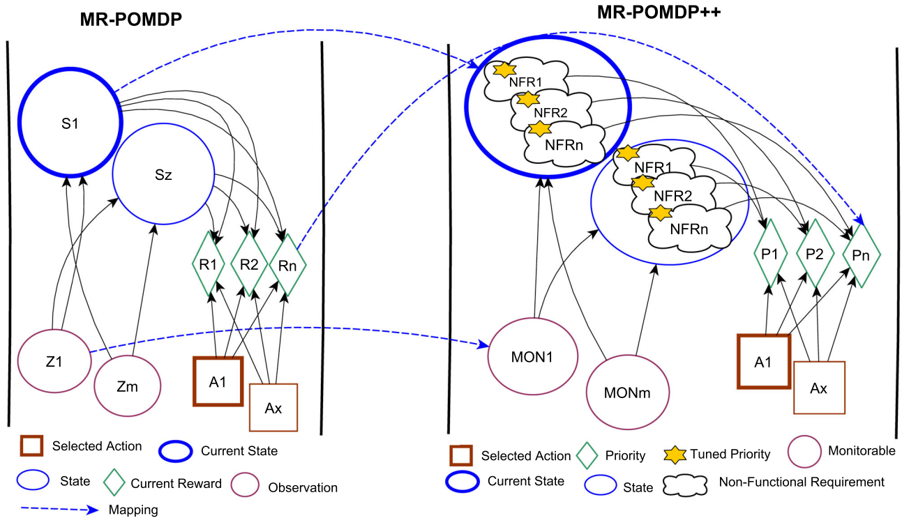
Fig. 5 Mapping of MR-POMDP to priority-aware MR-POMDP++
