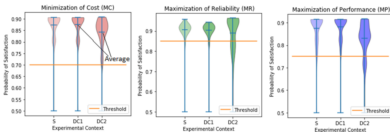
Fig. 16 Average satisfaction of NFRs under different environmental contexts—stable (S), detrimental context 1 (DC1) and detrimental context 2 (DC2)
