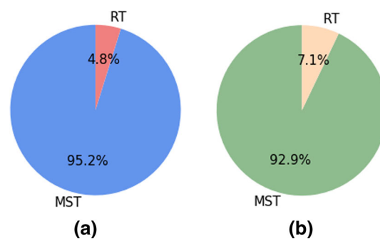
Fig. 13 Topologies selection under stable environmental context a Pri-AwaRE and b RE-STORM
