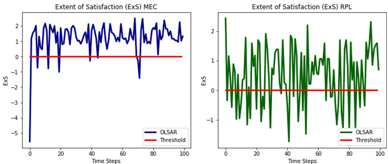
Fig. 9 Extent of satisfaction ( ExS ) of NFRs over time by applying Pri-AwaRE (using OLSAR)
