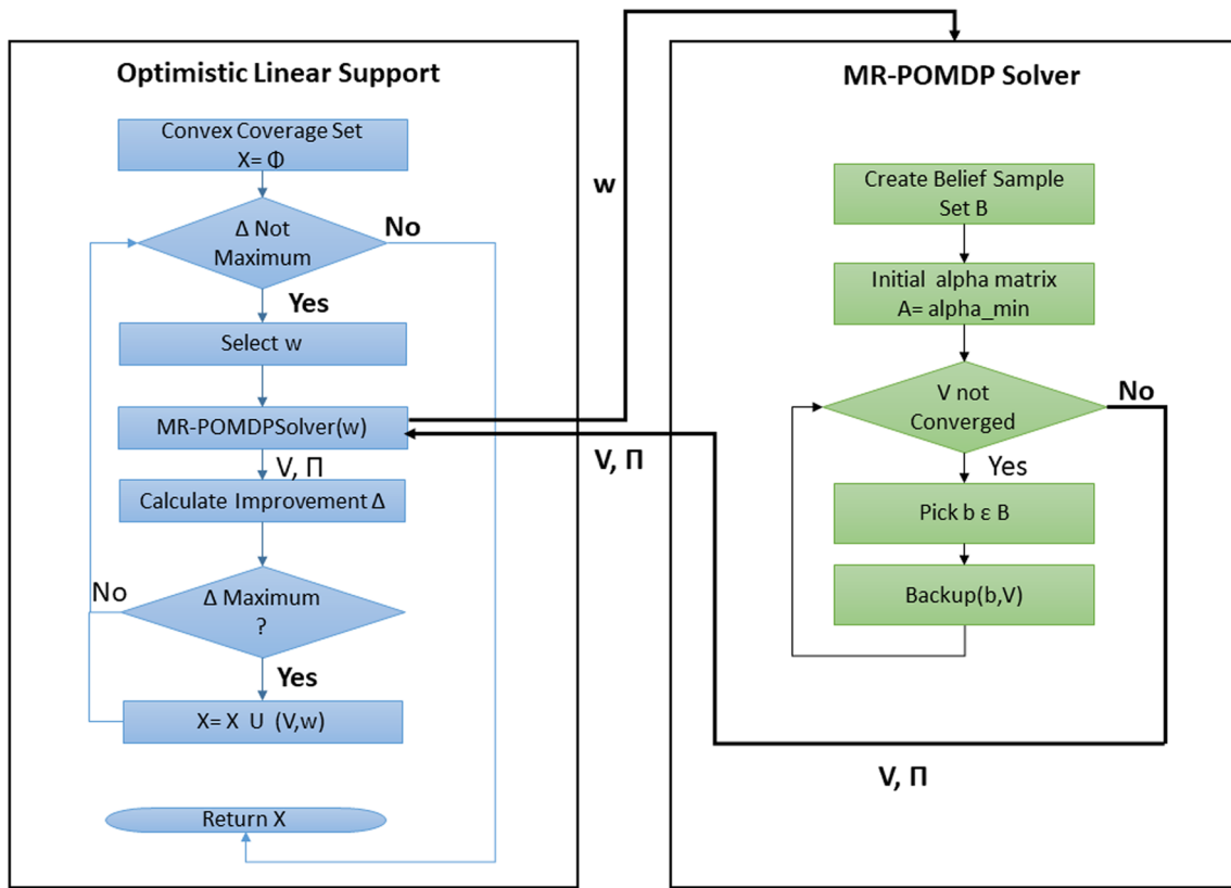
Fig. 4 Step By step execution of OLS
