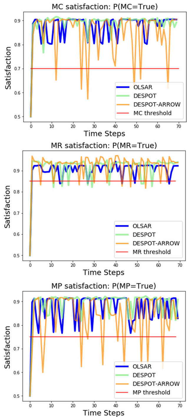
Fig. 11 Satisfaction of NFRs over time under detrimental context 1 (DC1) by applying Pri-AwaRE (using OLSAR), RE-STORM (using DESPOT) and RE-STORM-ARROW (using DESPOT-ARROW)
