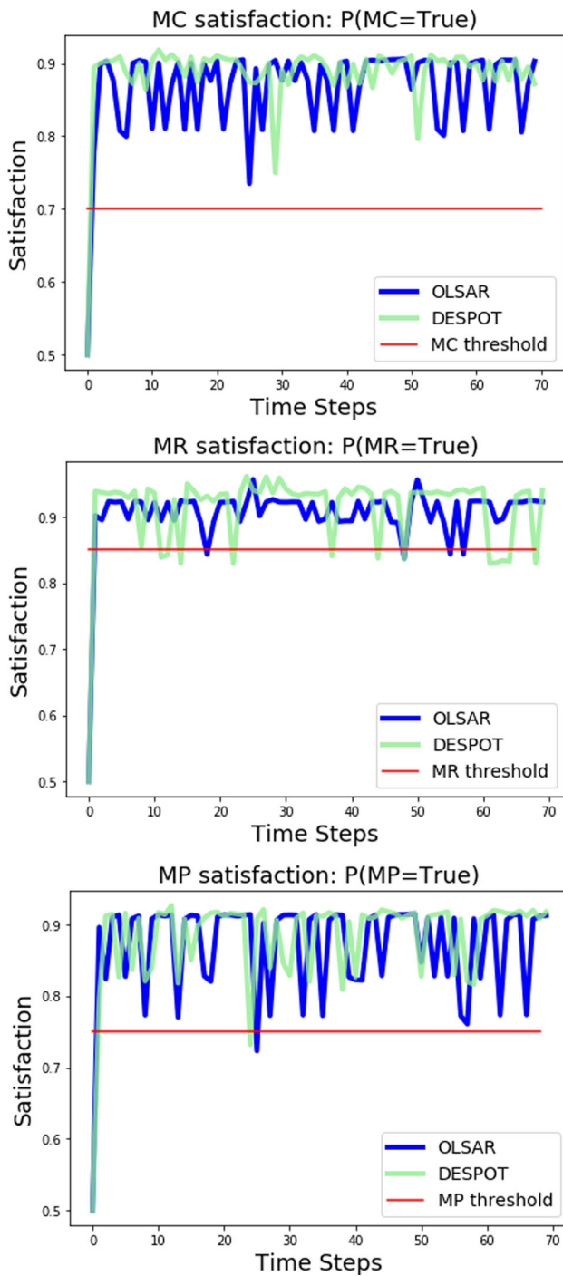
Fig. 10 Satisfaction of NFRs over time under stable conditions by applying Pri-AwaRE (using OLSAR) and RE-STORM (using DESPOT)
