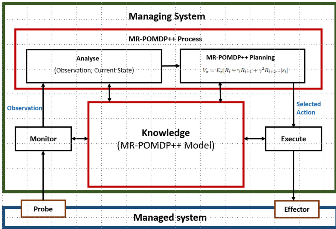
Fig. 6 Pri-AwaRE architecture
