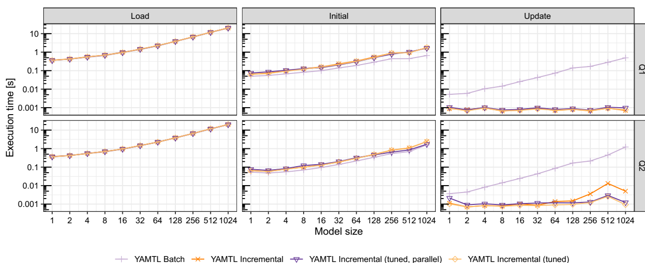
Fig. 18 Execution times of YAMTL solutions
