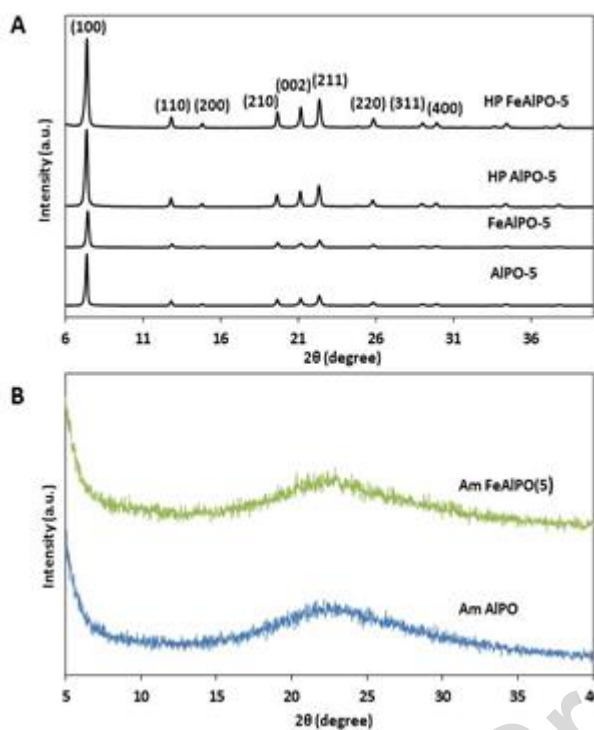
Figure 2. PXRD patterns of a) AFI aluminophosphates; b) amorphous aluminophosphates.
