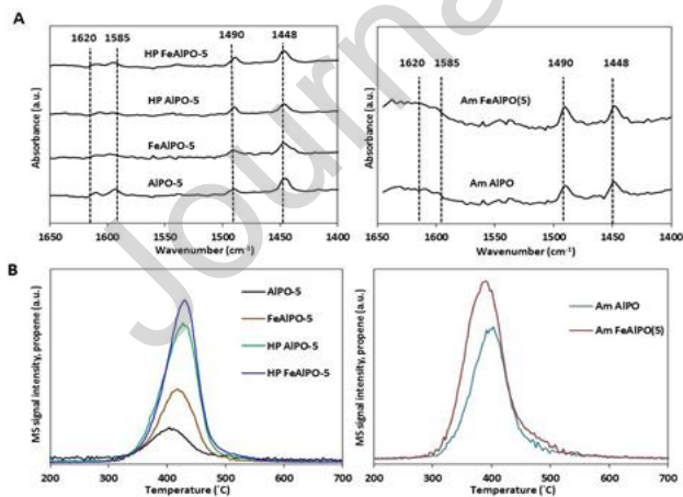
Figure 3. a) Pyridine probed DRIFT spectra; b) propylamine TPD-MS profiles of AFI aluminophosphates and amorphous aluminophosphates.
