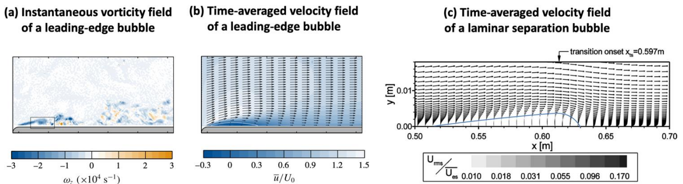
Figure 2 – Leading-edge bubble and laminar-separation bubble. The vorticity (a) and velocity field (b) of a leading-edge bubble measured by Stevenson et al. (2016) and the velocity field of a laminar-separation bubble (c) measured by McAuliffe & Yaras (2010).
