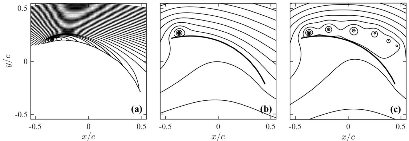
Figure 4 – The LEV computed and modelled on a horizontal section of an asymmetric spinnaker. The experimental time-averaged streamlines (a) measured by Arredondo-Galeana & Viola (2018); the complex potential model of the LEV when steady (b) and when unsteady (c).
