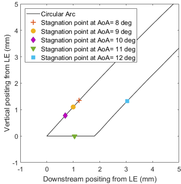
Figure 7 - Location of the stagnation point at the leading edge of a circular arc for different AoAs.
