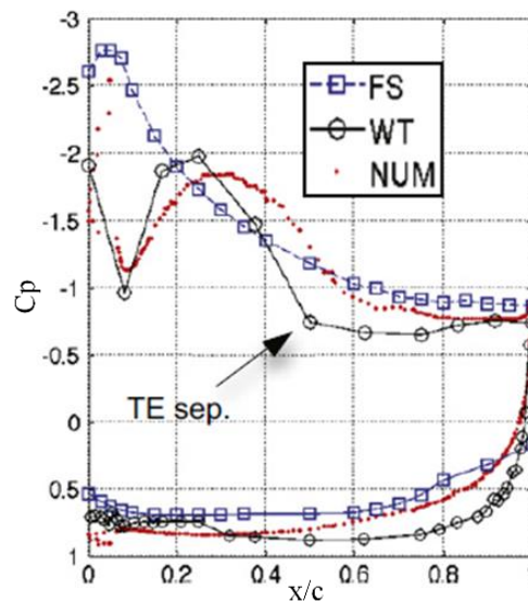
Figure 5 – Pressure distributions on the mid-span section of an asymmetric spinnaker , measured at full-scale (FS), in a wind tunnel (WT) and computed numerically (NUM) by Viola & Flay (2011).
