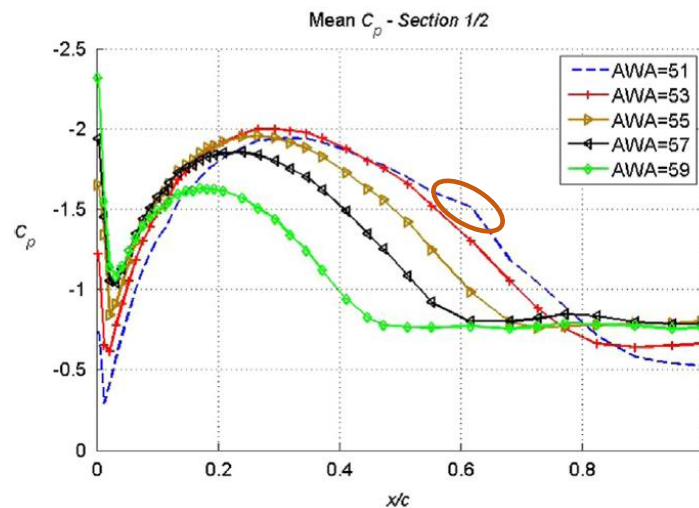
Figure 9 - Pressure coefficient along the mid-section of a spinnaker at different AoA (Bot et al , 2014).
