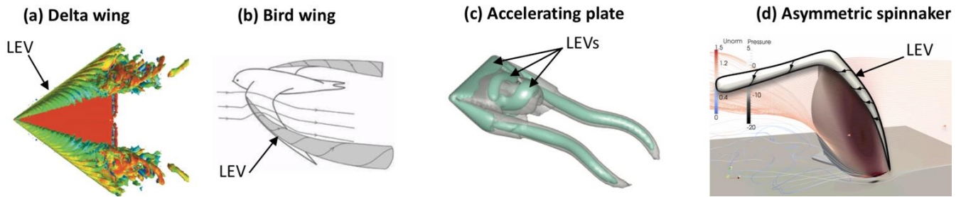
Figure 1 - The LEV on different lifting surfaces. (a) The steady LEV of a delta wing (Mitchell et al. , 2006); (b) the steady LEV on a gliding bird's wing (similar to the periodic LEV on flapping wings) (Videler et al. , 2004); (c) the unsteady LEV of an accelerating plate after having convected 5 chord lengths (Taira & Colonius, 2009); and (d) the intermittently steady LEV on an asymmetric spinnaker.
