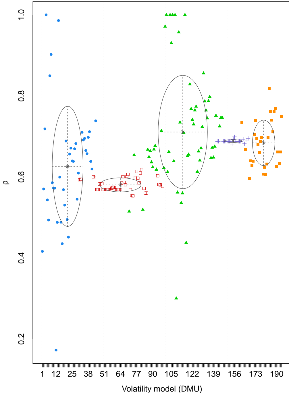
Figure 6: Cluster analysis plot for \rho
