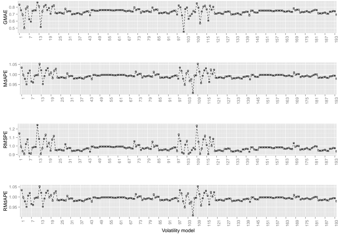
Figure 4: Line plots of GMAE, MdAPE, RMSPE and RMdAPE error measures
