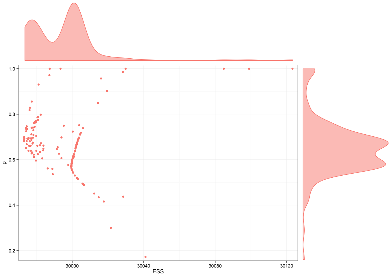
Figure 7: Joint density distributions of ESS and Efficiency scores ( \rho )
