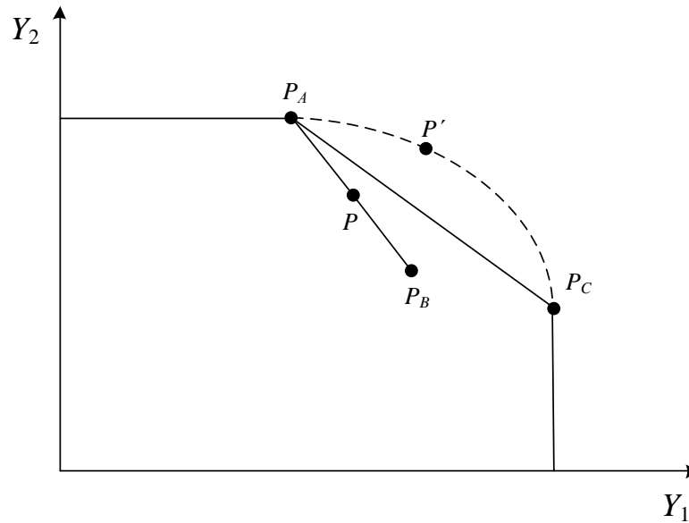
Figure 1: An output productivity possibility set.
