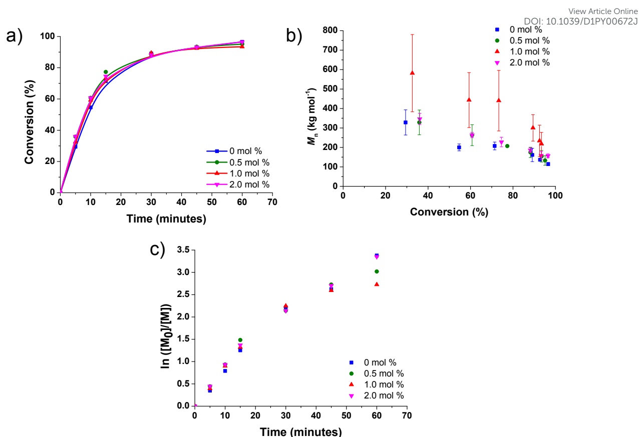
Figure 1. Kinetic data for the polymerisation of N,N -dimethylacrylamide (DMA) at varied bromoform content: (a) monomer conversion with time; (b) M_n versus monomer conversion; and (c) semi-logarithmic first-order plot.
