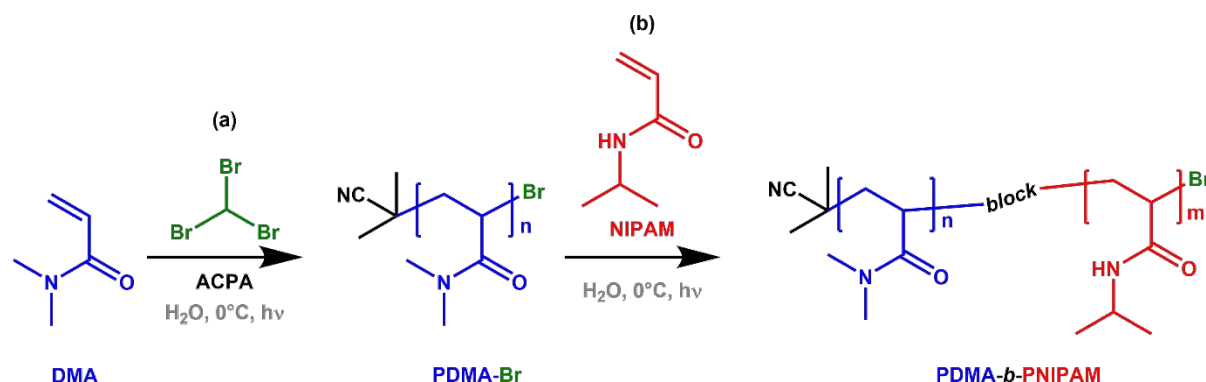
Scheme 1. (a) Step 1: Bromoform-assisted polymerisation of N,N -dimethylacrylamide (DMA). The proposed structure of the poly( N,N -dimethylacrylamide) macro-initiator (PDMA-Br) is based on the 4,4'-azobis(4-cyanopentanoic acid) (ACPA) radical fragment initiating the growth of a polymer chain and the bromoform-derived bromine radical ( \text{Br}^\bullet ) capping the chain-end. (b) Step 2: Polymerisation of N -isopropylacrylamide (NIPAM) using the PDMA-Br macro-initiator synthesised in Step 1 to produce poly( N,N -dimethylacrylamide)- b -poly( N -isopropylacrylamide) [PDMA- b -PNIPAM].
