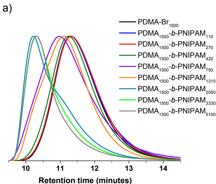
Figure 2. GPC traces of PDMA-Br macro-initiator and PDMA- b -PNIPAM copolymers with target PNIPAM DPs ranging from 170 to 6000
