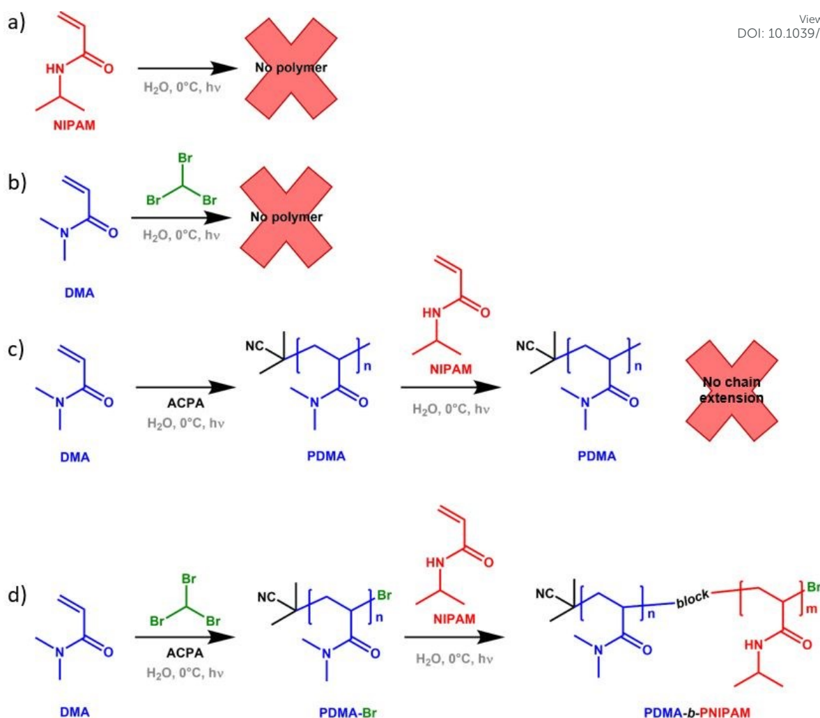
Scheme 2. (a) Attempted synthesis of PNIPAM homopolymer in the absence of bromoform and ACPA photoinitiator. (b) Attempted synthesis of PDMA homopolymer in the absence of ACPA photoinitiator. (c) Attempted synthesis of PDMA- b -PNIPAM copolymers without bromoform in Step 1. (d) Successful two step synthesis of PDMA- b -PNIPAM copolymers using PDMA prepared using bromoform in Step 1.
