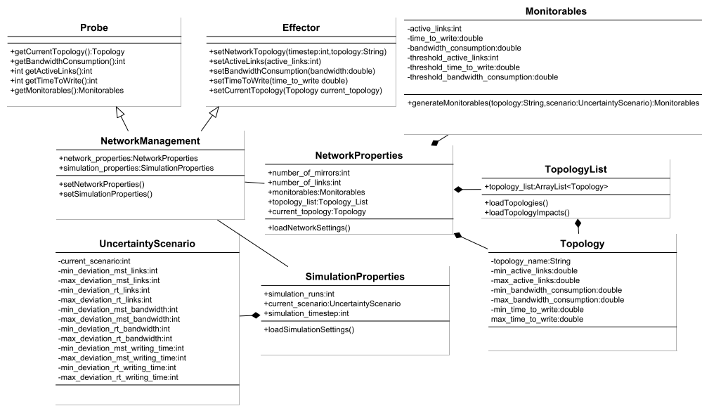
Fig. 2. RDMSim Class Diagram
