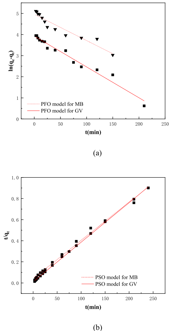
Fig. 2. PFO and PSO models plot for the adsorption of GV and MB onto SAC in single-component system.
