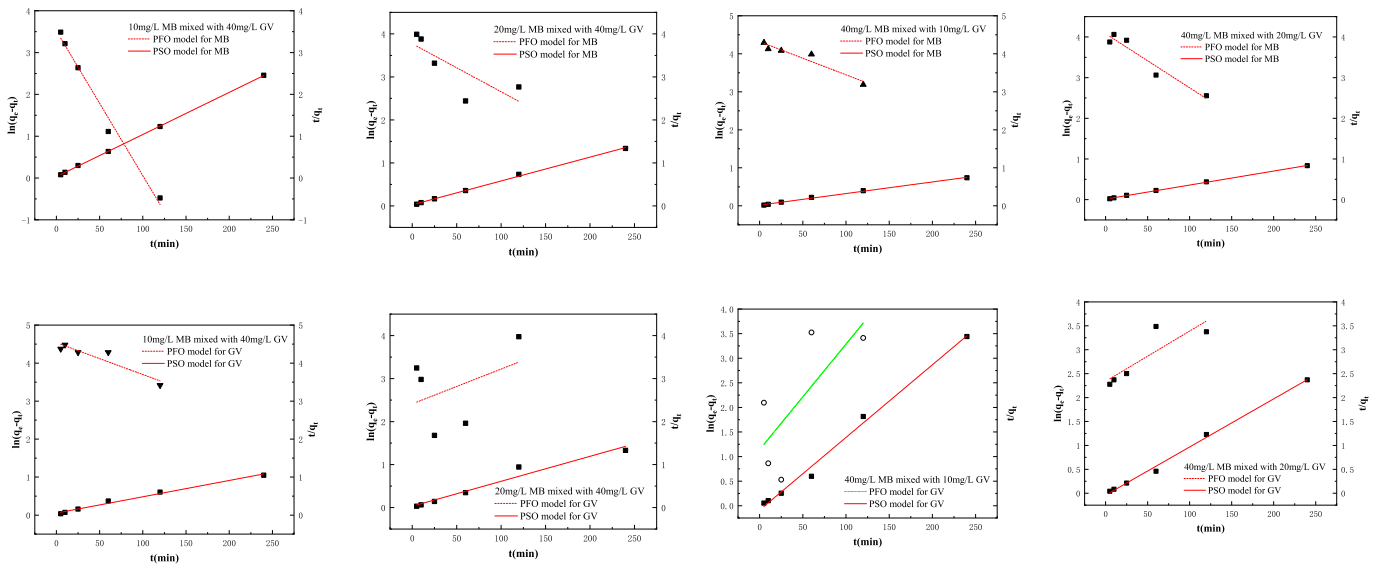
Fig. 3. PFO and PSO models plot for the adsorption of GV and MB onto SAC in two-component system.
