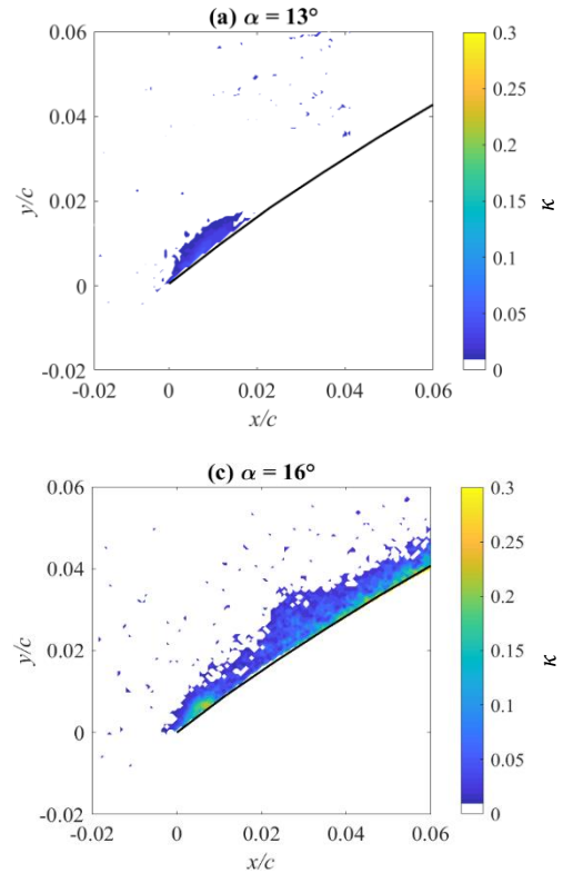
Figure 10. Nondimensional turbulent kinetic energy \kappa (plotted for \kappa > 0.01 ) at the leading edge pre ( \alpha = 13^\circ ) and post ( \alpha = 16^\circ ) critical angle of attack at Re = 68,200 .
