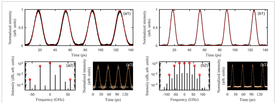
Figure 12. Besselon pulse trains generated at a repetition rate of 28 GHz with the phase-modulation depths (a) A_m = \pi/2 rad and (b) A_m = 3.72 rad. The temporal intensity profiles, optical power spectra and temporal profiles recorded in persistent mode are plotted in panels 1, 2 and 3, respectively. The experimental results (black curves) are compared with the theoretical predictions provided by (27) (red curves or circles). The horizontal white dashed lines in panel 3 indicate the zero-intensity level.
