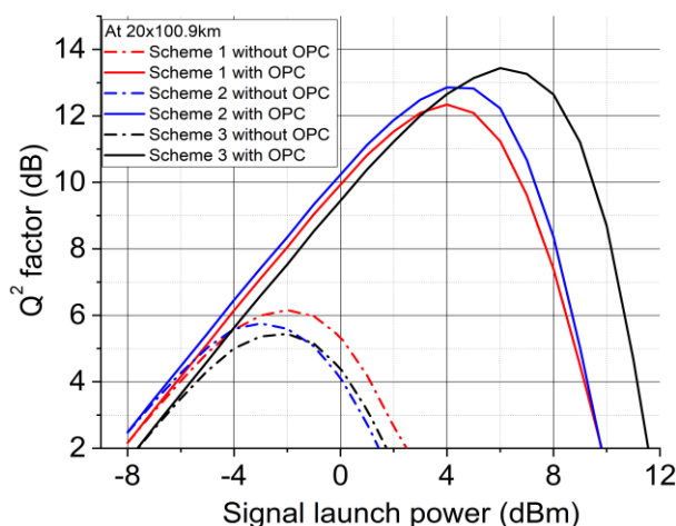
FIGURE 8. Simulated Q^2 factor versus signal launch power with/without OPC at ~2000km.
