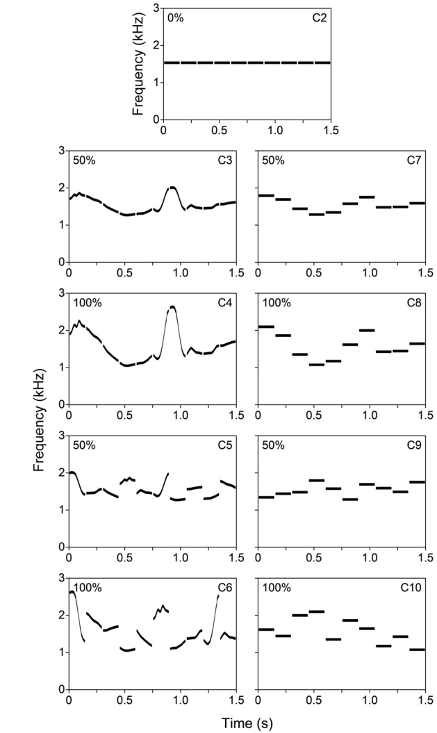
FIG. 3. Stimuli for experiment 2—schematic spectrograms illustrating formant-frequency contours and segmentation for the nine versions of the competitor derived from the example sentence “Mother ate the oranges” (conditions C2–C10). For all competitors, the constant amplitude contour was RMS-matched to the target F2 and divided into 150-ms-long segments; each segment was defined by raised-cosine amplitude ramps of \pm 10 ms. In each panel, the depth of the example F2C and the condition from which it was drawn are identified. The top panel (C2) illustrates the case where the F2C frequency contour was set to a constant value at the geometric mean frequency for the target F2 (constant segments, 0% depth). The four lower panels on the left (C3–C6) illustrate the versions of F2C in which the time-varying inverted F2 frequency contour was used after scaling it relative to that for the target F2 (50% or 100% depth) and the segments were presented either in the correct order or random order. The four lower panels on the right (C7–C10) differ from their counterparts on the left only in that each segment was set to a constant value at the geometric mean frequency for that segment.
