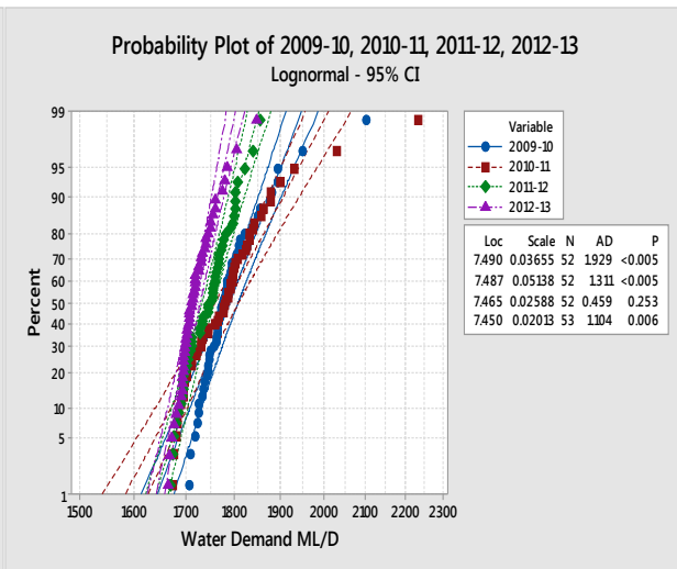
Fig. 2. Probability plots for Lognormal
