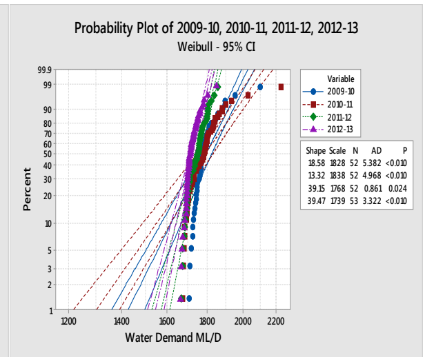
Fig. 4. Probability plots for Weibull
