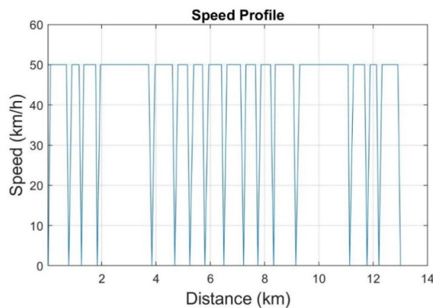
Figure 12. Speed profile of this vehicle vs. distance.
