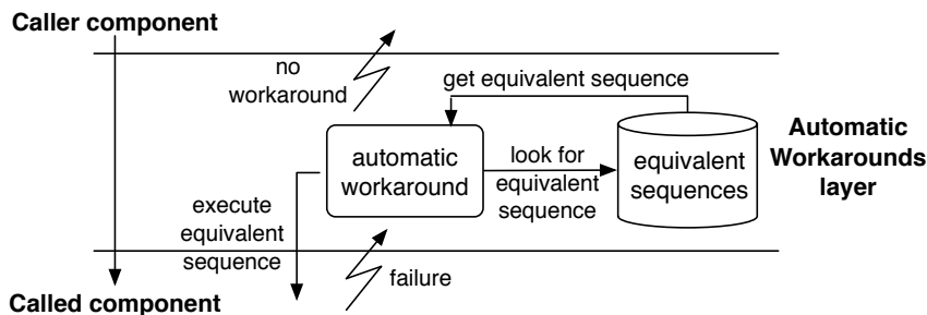
Fig. 2. The Automatic Workarounds technique
