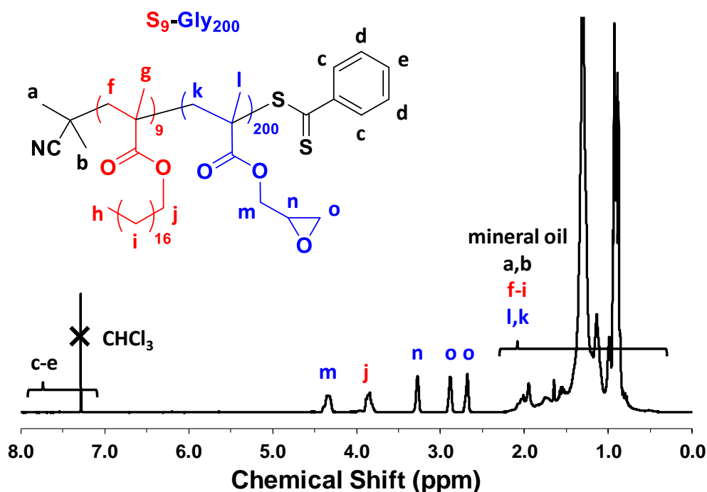
Figure 1. Assigned ^1\text{H} NMR spectrum recorded in \text{CDCl}_3 for a PSMA 9 -PGlyMA 200 ( S_9\text{-Gly}_{200} ) diblock copolymer after its synthesis via RAFT dispersion polymerization in mineral oil at 70 °C and 30% w/w solids. The signals labelled n, o and o indicate epoxy group survival.
