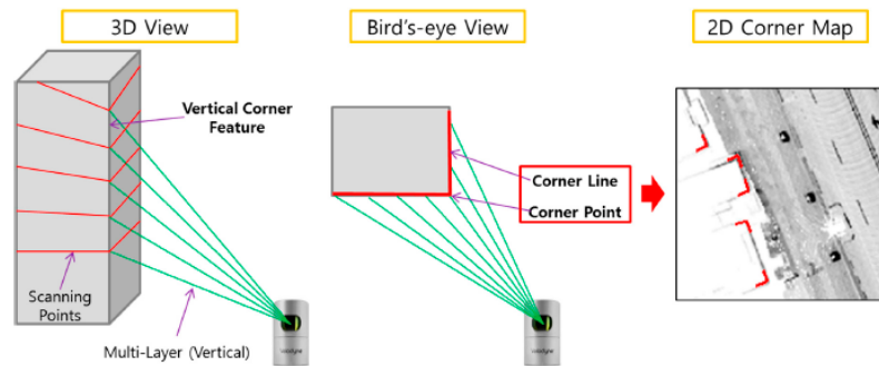
Figure 9. Corner definition in 3D and 2D systems [51].
