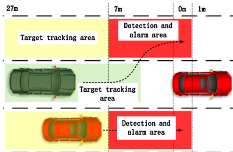
Figure 3. Bird-view of tracking pathway and blind area layout [22].
