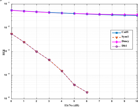
FIGURE 3. Wavelet-OFDM-MIMO-RoF system with diverse orthogonal wavelets
