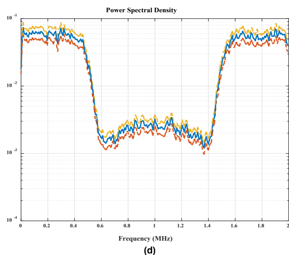
FIGURE 4. Power spectral density (PSD) spectra for the proposed system with 16-PSK modulation for (a) Transmitted signal (b) Received signal with db1/sym1 (c) Received signal with coif1 (d) Received signal with dmey wavelet.
