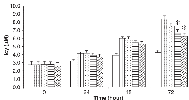
Fig. 3. Effect of adding folic acid on Hcy export. Bars indicate control (no methionine) and solutions with 100 \mu\text{M} methionine plus the addition of 0, 10, 100, and 1,000 nM folic acid (open, vertical striped, dotted, horizontal striped, and wavy bars, respectively). Results are derived from five experiments on three independent HUVEC cultures. Error bars denote standard deviations. Asterisks show significant differences from the 100 \mu\text{M} methionine, 0 nM folic acid value at P < 0.05 .
