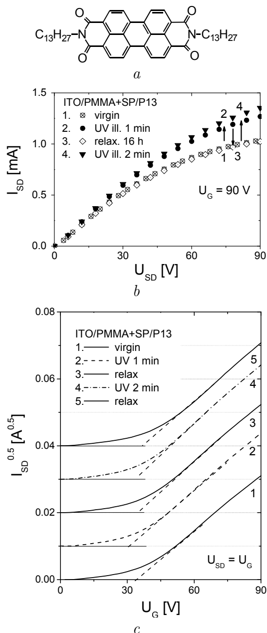
Fig. 7. Switching in the OFET consisting of n -type organic semiconductor N,N' -tridecylperylene-3,4,9,10-tetracarboxylic diimide (P13), and insulating PMMA containing 10 wt.% of photochromic spiropyran [22, 23]. (a) Chemical formula of the semiconductor. (b) An exemplary output current-voltage characteristics measured in the system demonstrating the switching. The sequence of measurements is indicated by arrows. (c) Locus ( U_{SD} = U_G ) current-voltage characteristics. The sequence of measurements is indicated in the diagram. To facilitate the comparison, curves 2–5 have been vertically displaced. The broken lines show linear fits to the experimental curves above the threshold voltages
