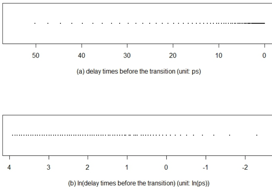
Figure 4.5: 76 different delay times before the transition - The figure shows 76 different delay times before the transition.
