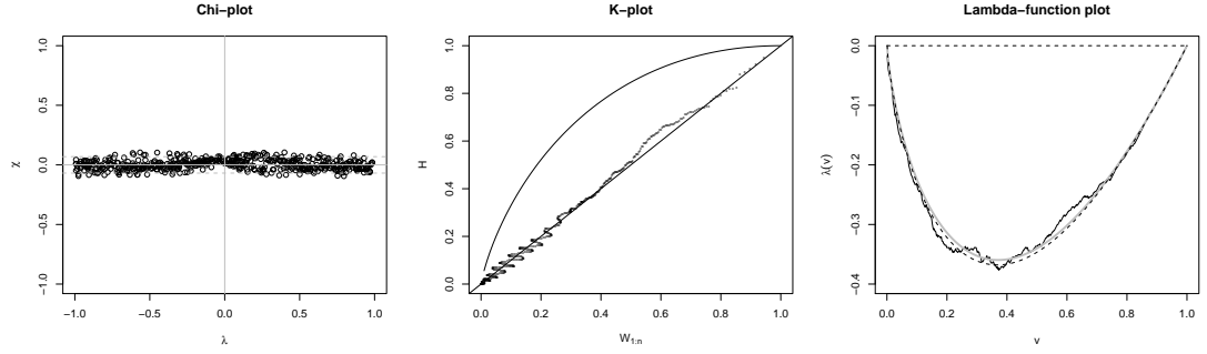
Figure 3.23: Chi-plot, K-plot and Lambda-function plot of angle dataset: edge 12 - The figure shows Chi-plot, K-plot and Lambda-function plot of angle dataset for edge: 12.
