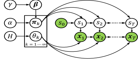
Fig. 1: The graphical model for the infinite HMM
