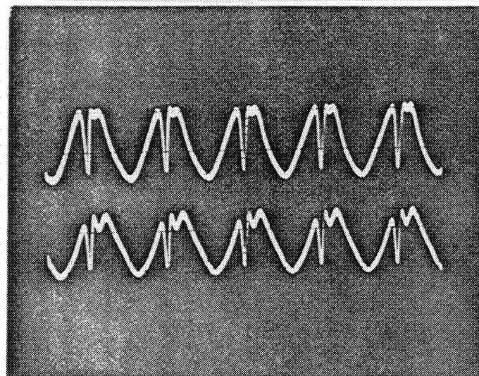
Fig. 5b. Demultiplexed signals (after low-pass filtering) for FBG's 3 and 4 with WDM and TDM.
