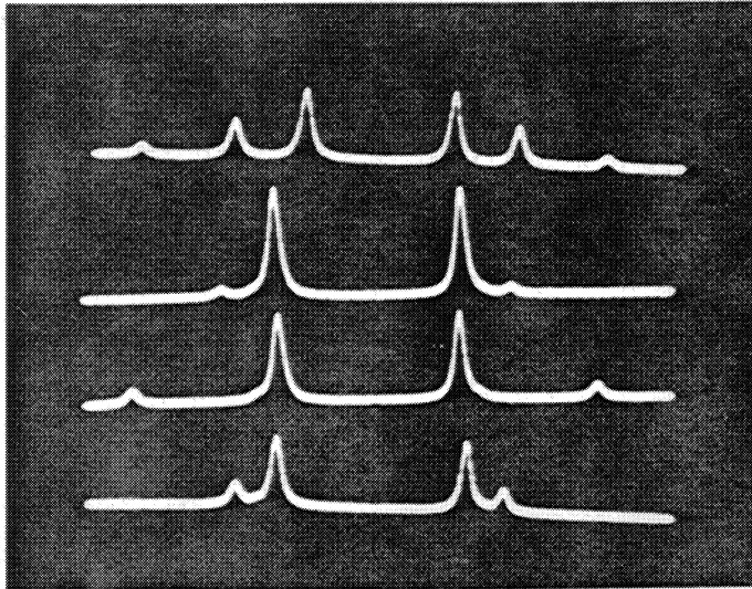
Fig. 4. Detected reflection spectra from FBG's 3 to 5 shown in the upper trace. Note that the waveform applied to the TWF is triangular, hence the traces repeat twice per scan.
