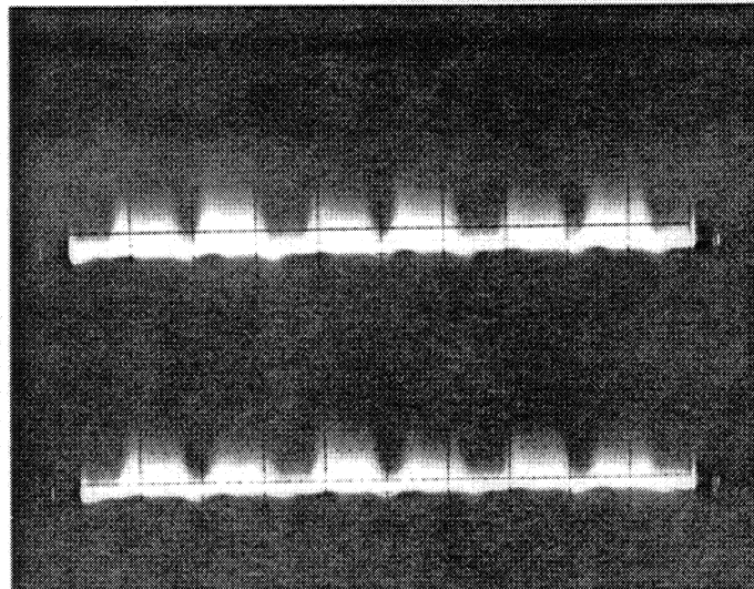
Fig. 5a. Photodetected return pulse signals. The top trace is pulses from FBG's 3 to 7 and the bottom trace is pulses from FBG's 8 to 11.
