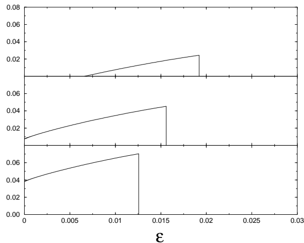
Figure 5. The complexity \Sigma(\epsilon) for (from top to bottom) p = 0.45 (below p_c ), p = 0.5 , and p = 0.55 (above p_c ); calculated for the case of a BEC and a (6, 3) regular code (Copied under permission from S. Franz, M. Leone, A. Montanari and F. Ricci-Tersenghi, The Dynamic Phase Transition for Decoding Algorithms, Phys. Rev. E 66 , 046120, (2002)[FLMRT02]. Copyright (2002) by the American Physical Society.).
