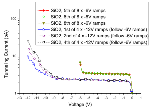
Fig.18. C-AFM I-V ramps on SiO 2 at bottom of etch pit, near Ti finger. Voltage is applied to the back-plane of the wafer.
