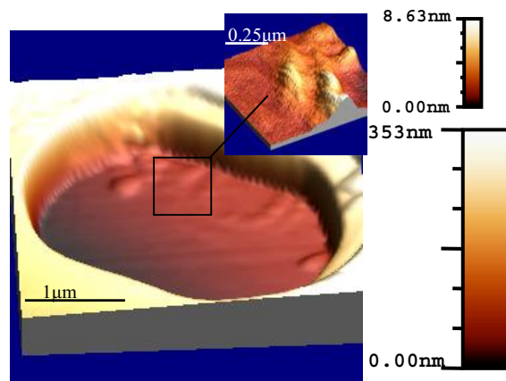
Fig.14. 3D topographical image of a 3x4 \mu\text{m} etch pit with discontinuous Ti finger (1x2 \mu\text{m} ) extending down and from edge of right hand long side of pit. See Fig.3 for schematic.
