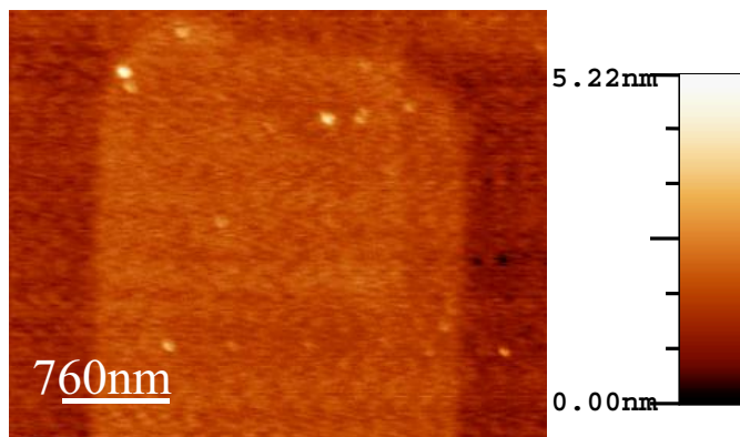
Fig.21. AFM topographical representation of the Ti finger inside the etch pit after 90% area oxidation. Breakdown spots can be seen on the finger and SiO 2 near the finger.
