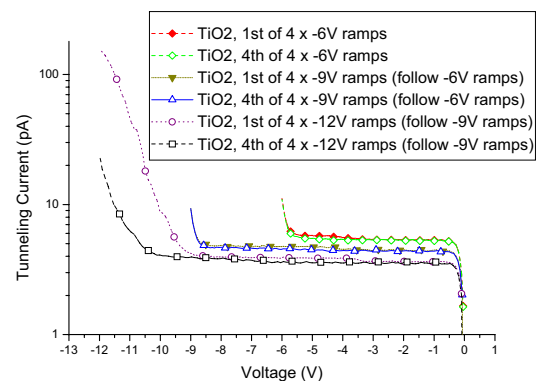
Fig.20. C-AFM I-V ramps on Ti finger, after repeated oxidation, at bottom of etch pit. Voltage is applied to the back-plane of the wafer.
