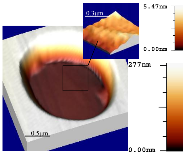
Fig.15. 3D topographical image of a 1.5x2 \mu\text{m} etch pit with discontinuous Ti finger (0.5x1 \mu\text{m} ) extending into it from edge of right hand long side.
