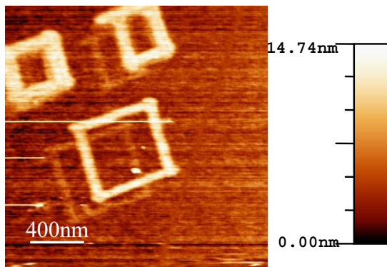
Fig.4. 0V tip bias topographic image of three squares anodically oxidized by AFM at 6V on a titanium surface.
