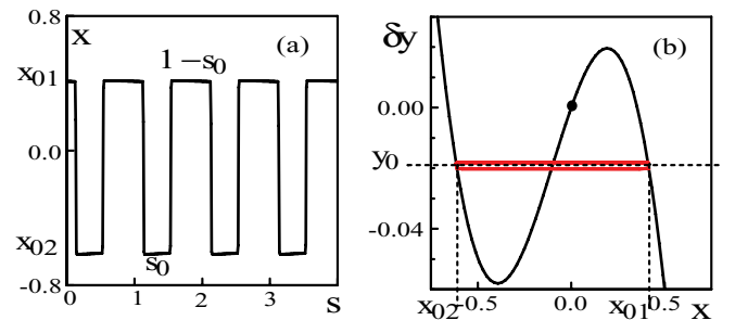
FIG. 2. (Color online) (a) Long time periodic solution obtained numerically from Eqs. (3) and (4). \varepsilon = 10^{-3} , \delta = 8.43 \times 10^{-3} , \Phi = -\pi/4 + 0.1 , \beta = 1.2 ; the initial conditions are x = -1 ( -1 \leq s < -1/3 ), x = 1 ( -1/3 \leq s < 0 ), and y(0) = 0 . (b) The periodic solution is represented in red (gray) in the phase plane (x, y) . The black line is the function (7), and the black dot is the unique steady state (x, y) = (0, 0) .
