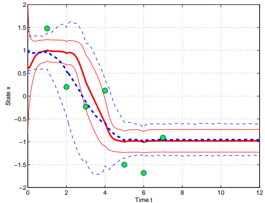
Fig. 2. The same as in Fig. 1 but with data set B (measurement noise variance = 0.36).
