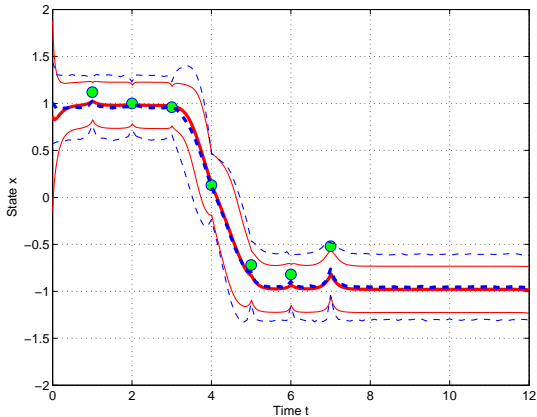
Fig. 1. Comparison of mean-path and conditional-variance estimates between the MCMC- (dashed) and variational (solid) method with a double-well potential system. Filled circles represent 7 observations from data set A , with measurement noise variance equal to 0.04. The mean paths are displayed by thick lines, while each pair of thin lines indicates an envelope of mean path with 2 \times standard deviation.
