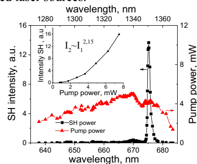
Fig.2. SHG power in 1/2-order of periodical poling (black squares) and pump power (red triangles) vs wavelength. Inset shows SHG power vs pump power.
