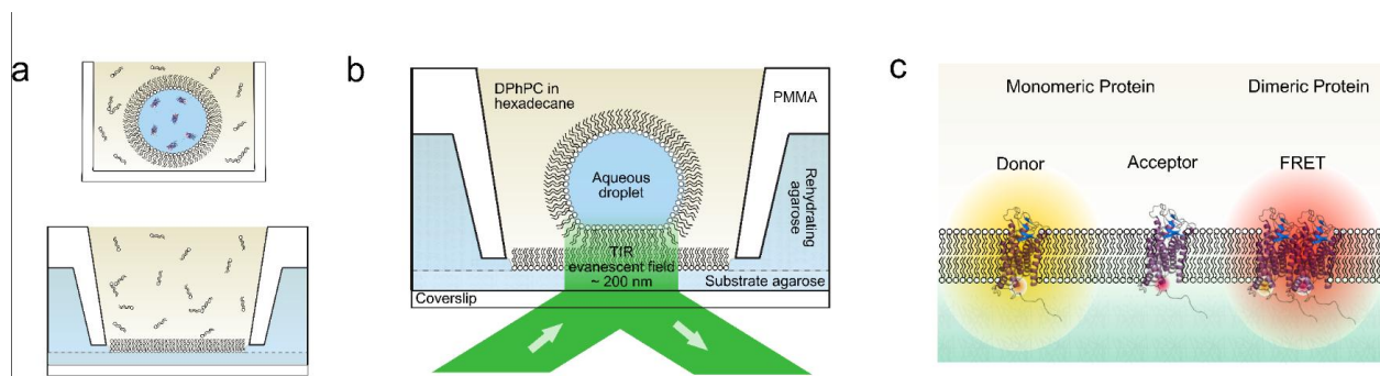
Figure 1: Single Molecule Imaging in droplet interface bilayers (DIBs): a) An agarose coated coverslip (bottom) and an aqueous droplet containing detergent stabilised protein (top) are separately incubated in lipid in alkane solution. A lipid monolayer spontaneously self-assembles at each water-oil interface. The aqueous droplet is subsequently transferred into the well of the PMMA device housing the agarose-coated coverslip substrate. b) A lipid bilayer forms on the contacting of the two self-assembled monolayers of the droplet and agarose layer. Purified membrane proteins present in the droplet integrate into the resultant bilayer. Total internal reflection of laser light at the glass-sample interface generates an evanescent field illuminating the membrane enabling fluorescent imaging. c) Total internal reflection fluorescence (TIRF) enables single molecule imaging of membrane proteins reconstituted into DIBs. This schematic illustrates the use of single molecule FRET to image donor-labeled monomeric protein and FRET-capable donor and acceptor labeled dimeric protein complexes at the single molecule level. An approach adopted to elucidate the dimerisation dynamics of the GPCR, NTS1, in DIBs [56].
