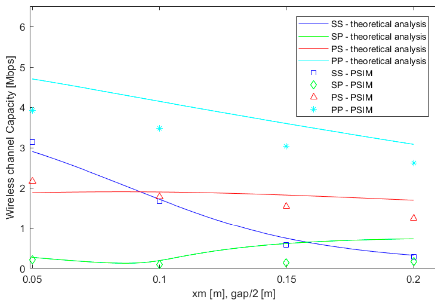
Figure 6. Variations in the wireless channel capacity due to vertical and horizontal misalignments.
