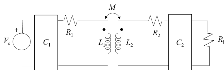
Figure 2. Equivalent circuit of an ICPT system.
