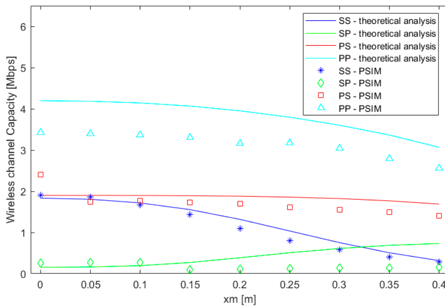
Figure 5. Variations in the wireless channel capacity due to horizontal misalignments.
