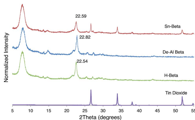
Fig. 1 X-ray diffractograms of tin dioxide, H-beta, De-Al-beta, and Sn-beta.
