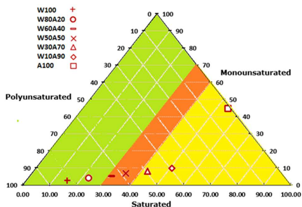
Fig. 4 Analyses of biodiesels according to their degree of unsaturation. Zones satisfying parameters for EN 14214 norms; green area satisfies the viscosity at 40 °C; yellow area satisfies the iodine number; orange area satisfies both viscosity and iodine number
