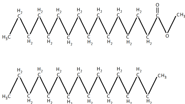
Fig. 1 Typical biodiesel molecule vs petroleum molecule diesel, adapted from [6]
