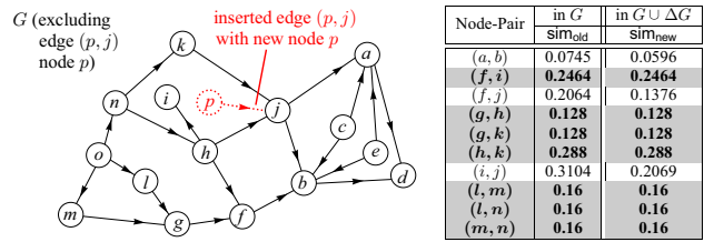
Fig. 4 Incrementally update SimRank when a new edge (p, j) with p \notin V and j \in V is inserted into G = (V, E)
