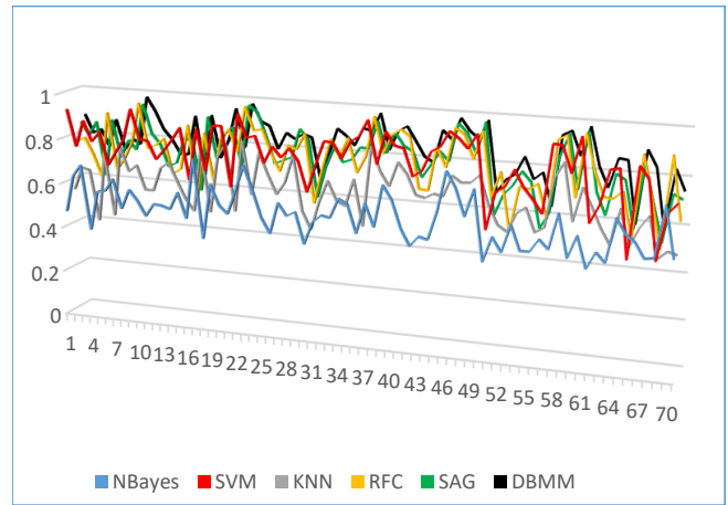
Fig. 6: Results of the 70 tests for the KDEF dataset in terms of F-Measure. We can see that the DBMM has a consistent performance when compared to its base classifiers.
