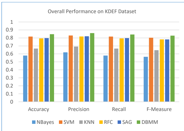
Fig. 5: Results for the KDEF dataset in terms of accuracy, precision, recall and F-Measure. Average of all 70 tests (leave-one-out cross-validation on unseen person).
