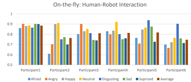
Fig. 7: Tests on-the-fly using the robot NAO. The KDEF dataset was used for training, and 6 new (unseen) subjects, 4 males and 2 females, participated in a human-robot interaction task, performing the emotional expressions. For the on-the fly tests the overall accuracy (average) was 80.6%
