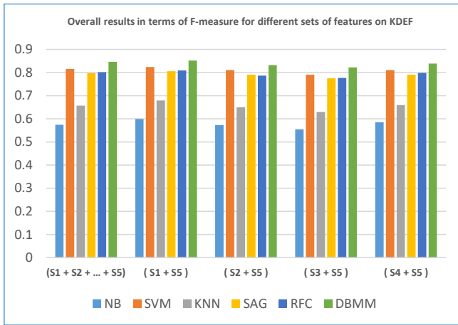
Fig. 4: Overall results in terms of F-measure for all subsets of features on KDEF dataset.
