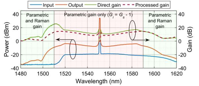
Fig. 2. Experimental demonstration of signal-idler mixing (fiber length 100 m, pump wavelength 1551 nm, pump power 2 W). Wavelength ranges corresponding to different idler gains are highlighted. Direct gain (green curve) is found as a ratio between measured output (orange curve) and input (blue curve) spectra. Processed gain (broken red curve) is found using (2) and the same output and input spectra.
