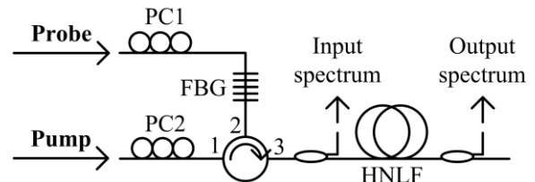
Fig. 1. Generalized FOPA experimental setup for gain spectrum characterization using a narrowband or broadband probe.
