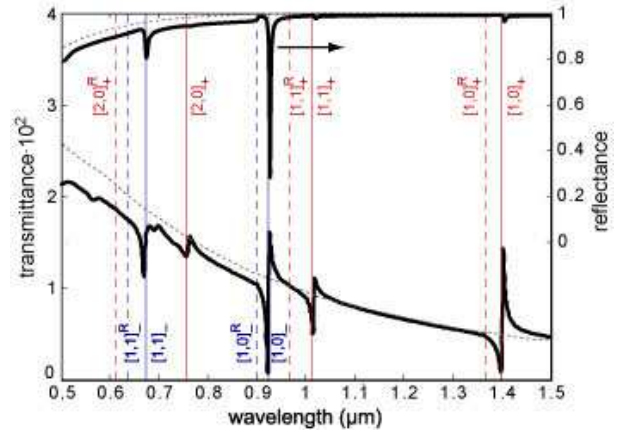
FIG. 5: (Color online) Dependence of transmittance and reflectance upon the wavelength for the wave normally-incident from the air superstrate onto the silver film bounding with the quartz substrate. The parameters of C_{4v} array, are \rho_1 = \rho_2 = \rho = 0.9\mu m , a/\rho = 1/3 . The incident wave electric field \mathbf{E} is parallel to \mathbf{g}_1 (to Ox axis, see. Fig. 1). The inclusion impedance, \xi_i , is taken to be \xi_i = 2\xi_f . The film thickness is equal to 2.3 skin depths. The transmittance and reflectance of the unmodulated film are plotted with dotted lines. The vertical solid and dashed lines indicate the wavelengths relevant to SPPs on the unmodulated boundaries and Rayleigh points respectively.
