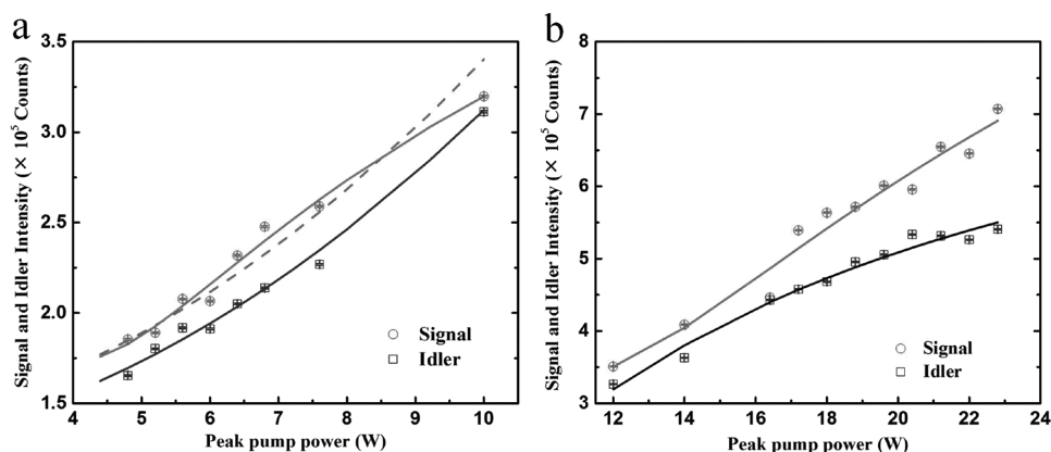
Figure 4. The signal and idler counts as a function of peak pump power per 1.7 min; a) < 11\text{ W} and b) > 11\text{ W} . Circle (square): the signal (idler) from the SWNTs. In (a), blue, red dashed, and green lines are the fitting results of N_i for the idler, N_s , and N_s^i (green line) for the signal, respectively. In (b), the fitting curve of N_i^i (black line) is for the idler, and N_s^i (green line) for the signal. Error bars for each data point are included.
