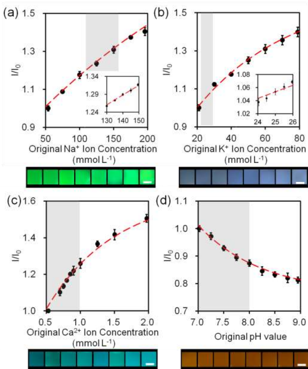
Figure 7. Quantifications of electrolytes in artificial tear fluid using the smartphone readout system: (a) Na + ions, (b) K + ions, (c) Ca 2+ ions and (d) H + ions sensing readout by ImageJ. Scale bars: 2 mm. Insets in (a) and (b) show Na + ion concentration in the range of 130-150 mmol L -1 and K + ion concentration in the range of 24-26 mmol L -1 . Error bars represent standard deviation ( n=3 ). Curves (red dashes) were fitted using Eq. 3. Shadows show the physiological Na + , K + , Ca 2+ ion and pH range.
