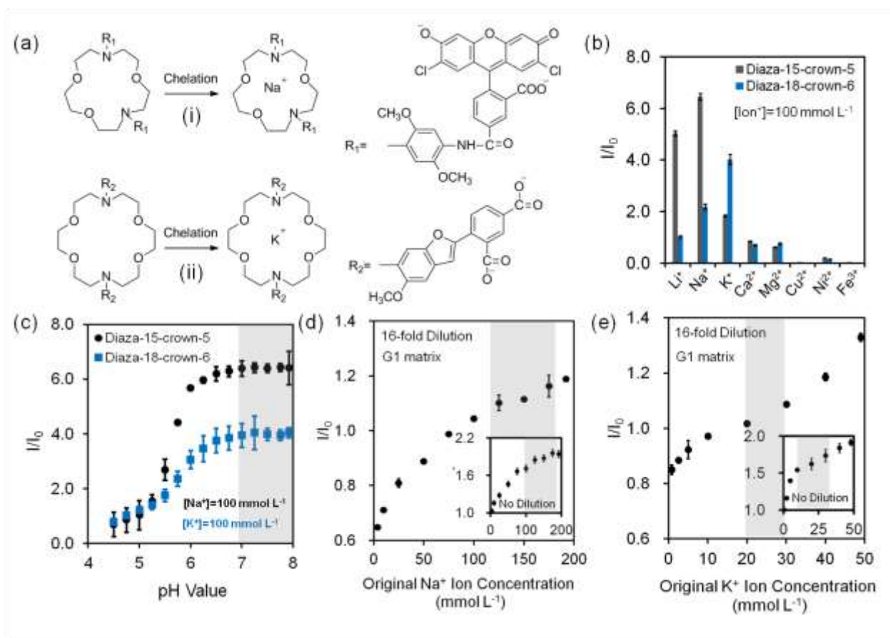
Figure 3. Na + and K + ion measurements using fluorescent crown ether derivatives in buffer solutions (tris, pH 7.4, 150.0 mmol L -1 ). (a) Chelation mechanisms of fluorescent (i) diaza-15-crown-5 and (ii) diaza-18-crown-6 with monovalent metal ions. (b) Selectivities of diaza-15-crown-5 and diaza-18-crown-6 (25 μmol L -1 ) for mono/divalent ions (100.0 mmol L -1 ) in aqueous solutions. (c) The effect of pH on fluorescence readouts at constant Na + and K + ions (100.0 mmol L -1 ) and diaza-15-crown-5 and diaza-18-crown-6 (25 μmol L -1 ) concentrations in aqueous solutions. Quantifications of 16-fold diluted (d) Na + and (e) K + ions on G1 matrix at a constant probe concentration (25 μmol L -1 ). Insets show the quantifications of non-diluted Na + and K + ions on G1 matrix. Error bars represent the standard deviation (n=3). Shadows in Fig. 3c-e show the physiological pH, Na + ion and K + ion range.
