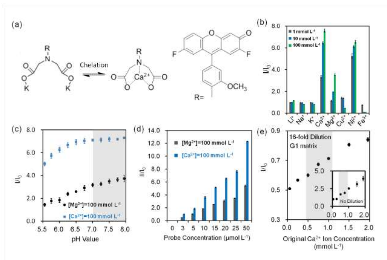
Figure 4. Quantification of divalent metal ions in buffer solution (tris, pH 7.4, 150.0 mmol L -1 ) at 25 °C. (a) Chelation mechanism of o -acetanisidide with divalent metal ions. (b) Fluorescence readouts of o -acetanisidide in the presence mono/divalent metal ions in aqueous solutions. (c) The effect of pH on fluorescence readouts of o -acetanisidide (25 μmol L -1 ) at constant Mg 2+ and Ca 2+ ion concentrations (100.0 mmol L -1 ) in aqueous solutions. (d) Fluorescence intensity readouts of Mg 2+ and Ca 2+ ions (100 mmol L -1 ) as the concentration of o -acetanisidide were varied from 3-50 μmol L -1 . (e) Quantification of 16-fold diluted Ca 2+ ions on G1 matrix at a constant o -acetanisidide concentration (25 μmol L -1 ) in aqueous solutions. Insets show the quantification of non-diluted Ca 2+ ions on G1 matrix. Error bars represent the standard deviation (n=3). Shadows in Fig. 4c and 4e show the physiological pH and Ca 2+ ion range.
