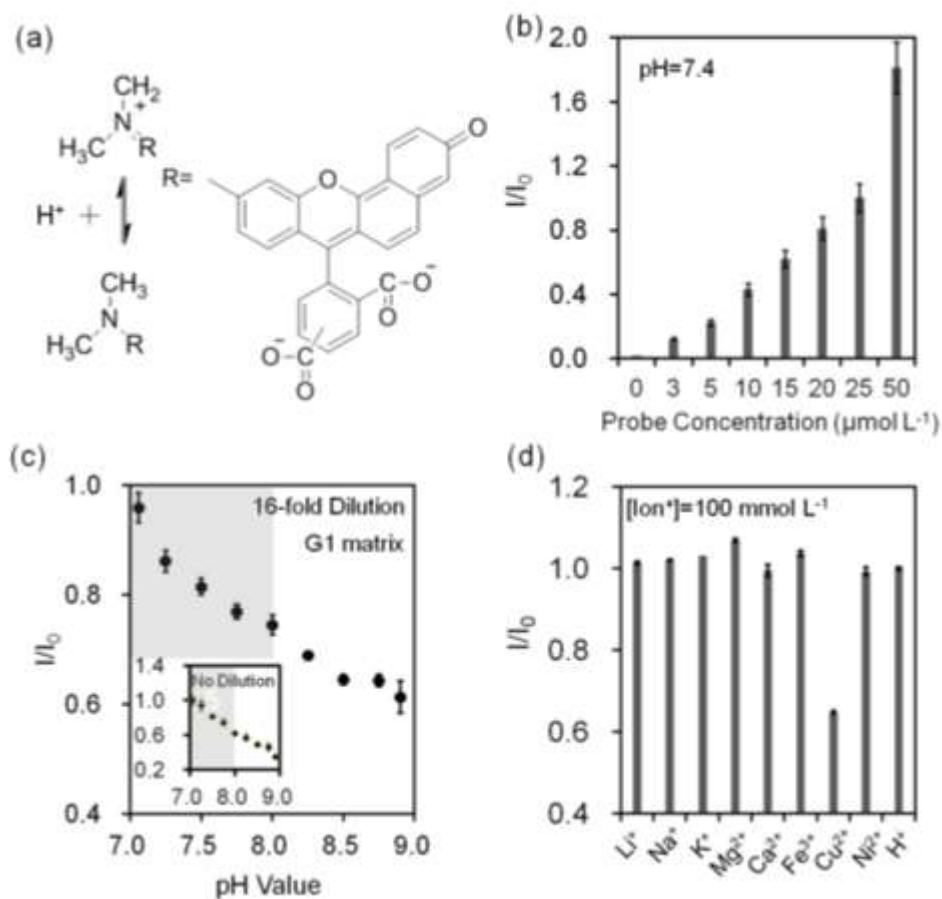
Figure 5. Quantification of pH values in buffer solutions (tris, 150.0 mmol L -1 ) at 25 °C. (a) Principle of operation of seminaphtorhodafluor. (b) Fluorescence intensity readouts as the concentration of seminaphtorhodafluor was varied from 3-50 μmol L -1 at pH=7.4 in aqueous solutions. (c) Quantification of tris buffer pH (inset) and 16-fold diluted tris buffer (150.0 mmol L -1 , pH=7.4) on G1 matrix at a constant seminaphtorhodafluor concentration (25 μmol L -1 ). (d) Relative fluorescence intensity readouts of mono/divalent ions at a constant concentration of seminaphtorhodafluor (25 μmol L -1 ) at pH 7.4. Error bars represent standard deviation (n=3) in aqueous solutions. Shadows in Fig. 5c show the physiological pH range.
